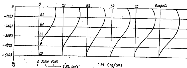
図-14 M (kg/cm)
