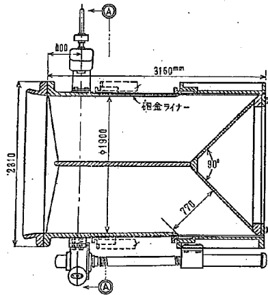
附図-3 HOWELL-BUNGER VALVE DETAILS
