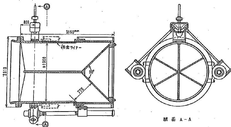
附図—3 HOWELL-BUNGER VALVE DETAILS
