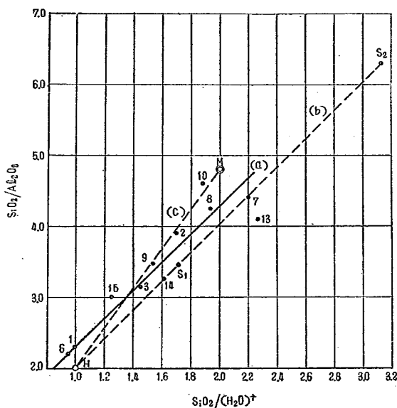
図-7 \text{SiO}_2/\text{Al}_2\text{O}_3 と \text{SiO}_2/(\text{H}_2\text{O})^+ の関係
