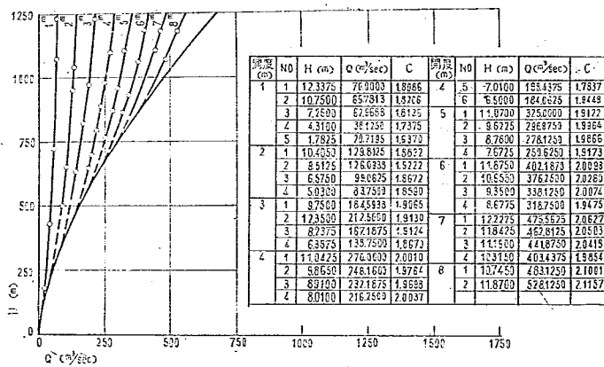
H-Q GATE 1 図-69 1門等高半開
