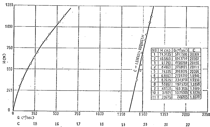
H-Q H-C GATE 2
