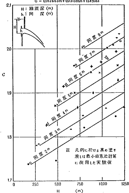
H-C GATE 2 図-68 1門等高半開
