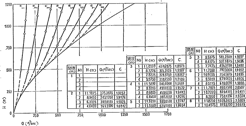
図-61 2門等高半開
