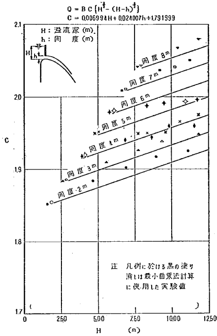
H-C GATE 2, 3 図-62 2門等高半開
