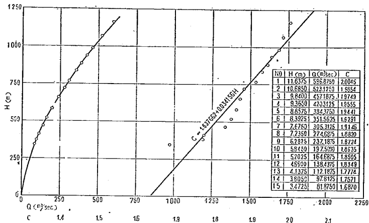
H-Q H-C GATE 1
