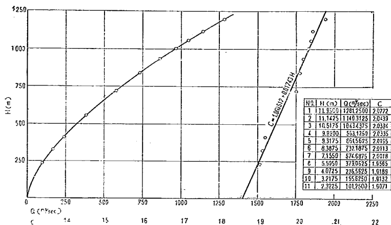
H-Q H-C GATE 2, 3
