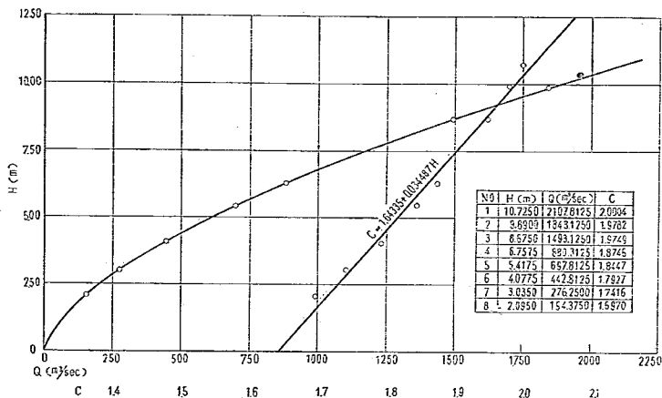
H-Q H-C GATE 1, 2, 3, 4
