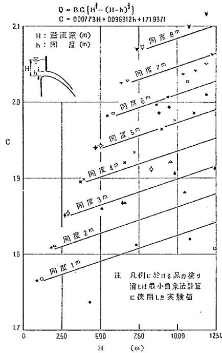
H-C GATE 1 図-70 1門等高半開
