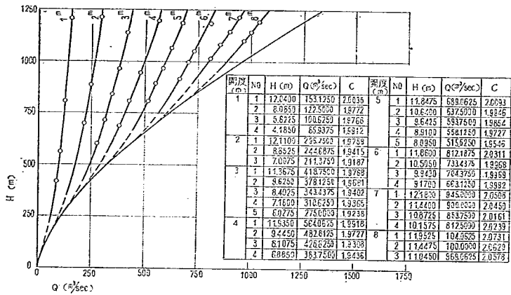
H-Q GATE 1, 3 図-63 2門等高半開
