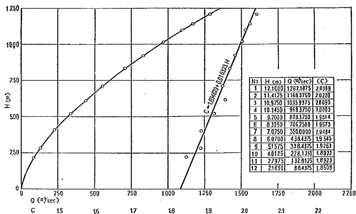
H-Q H-C GATE 1, 4
