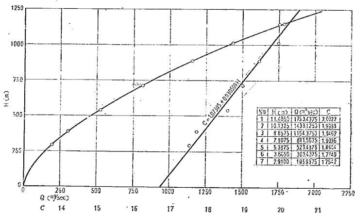
H-Q H-C GATE 1, 2, 3
