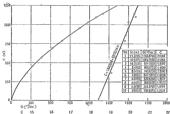
H-Q H-C GATE 1, 3
