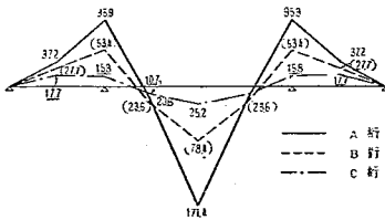
たわみ図 (1/100mm) P = 22 \times 9
