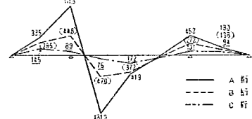
たわみ図 (1/100mm) P = 22 \times 9
