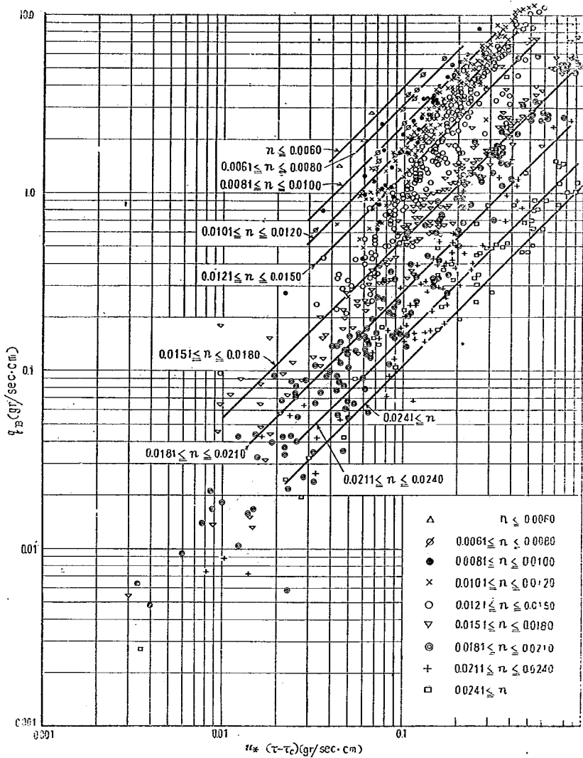
図-5 q_B \sim u_{*s}(\tau - \tau_c)
