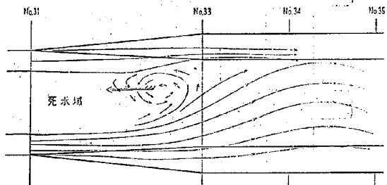
図-11 流況図(B案)
