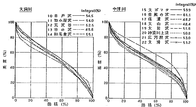
図-23 (2) hypsometric curve
