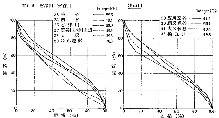
図-23 (3) hypsometric curve
