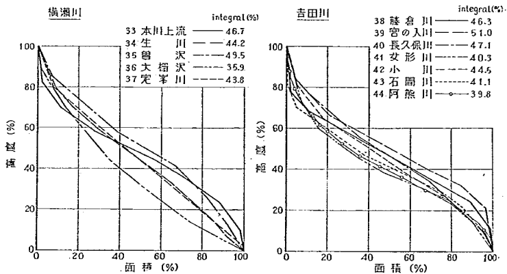
図-23 (4) hypsometric curve
