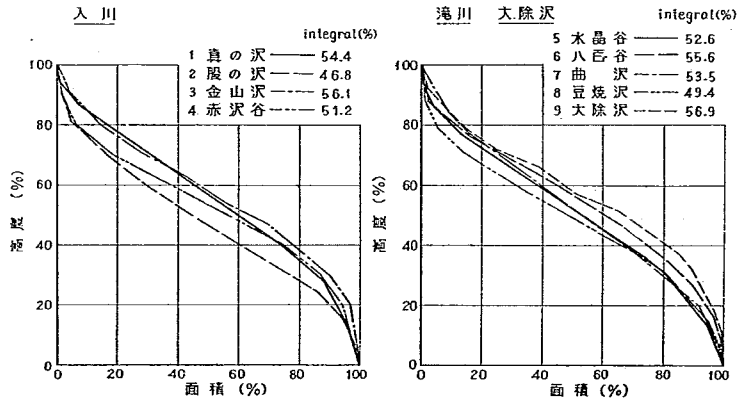
図-23 (1) hypsometric curve
