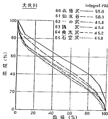
図-23 (6) hypsometric curve
