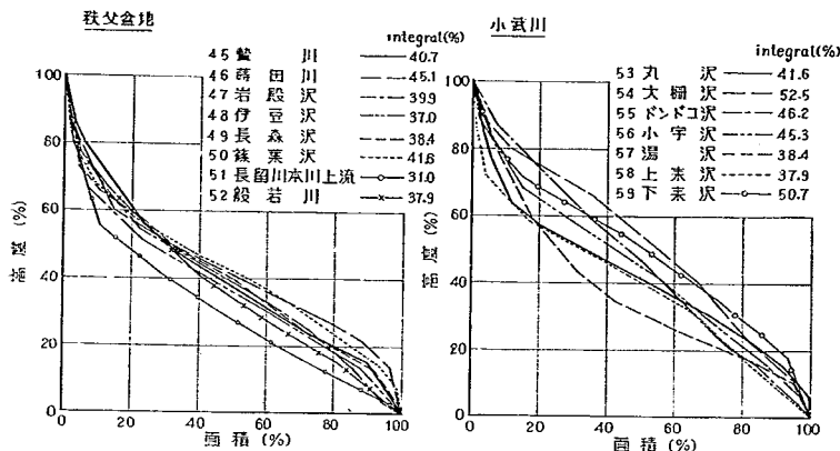
図-23 (5) hypsometric curve
