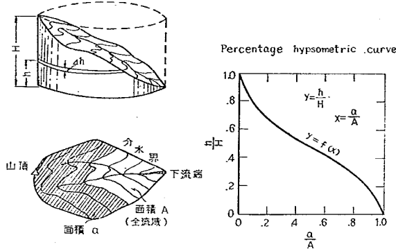
図-3 hypsometric curve
