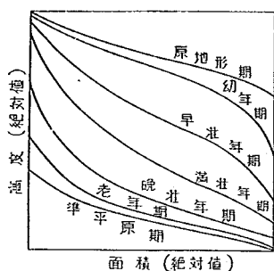
図-20 侵食 stage と hypsometric curve
