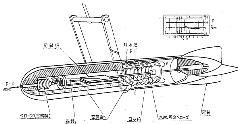
図-7 III型水深流速計
