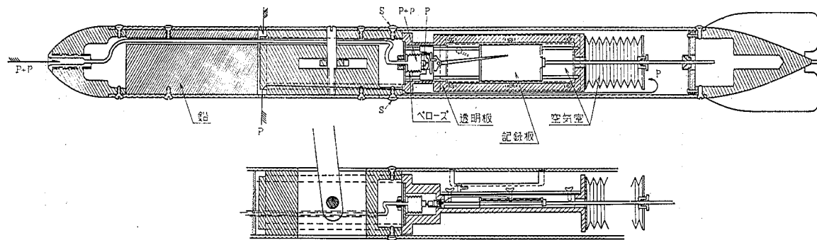
図-6 III型水深流速計
