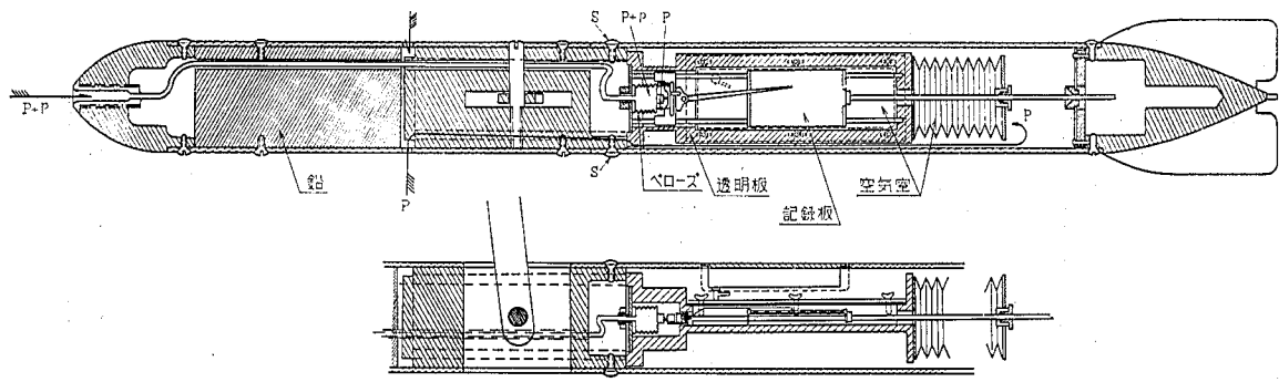
図-6 III型水深流速計
