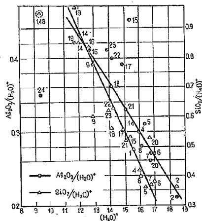
図-13 \text{Al}_2\text{O}_3/(\text{H}_2\text{O})^+ , \text{SiO}_2/(\text{H}_2\text{O})^+ と (\text{H}_2\text{O})^+ の関係
