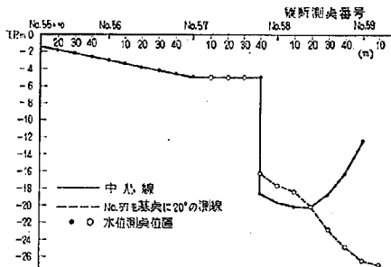
図-1 2-12型, 2-13型, 2-14型模型河床縦断
