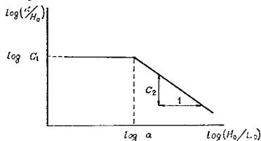
図-5 R/H_0 \sim H_0/L_0
