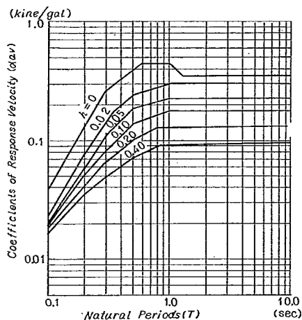
Spectrum Curves Coefficients of Response Velocity
