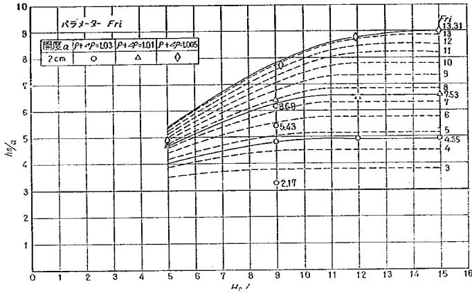
図-5.6 Q_e/Q=0.8 h_0/a \sim H_2/a
