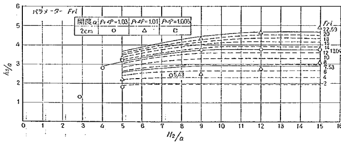
図-5.4 Q_2/Q=0.2 h_1/a \sim H_2/a
