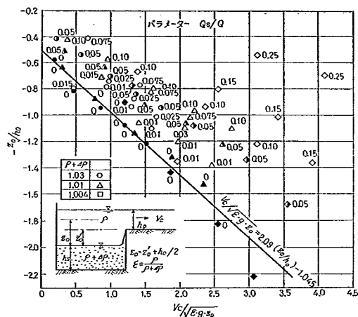
図-5.10 -Z_0/h_0 \sim V_c/\sqrt{\epsilon g s_0}
