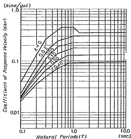
図-6 Spectrum Curves Coefficients of Response Velocity
