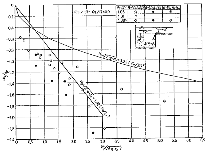
図-5.13 -Z_0/h_0 \sim V_c/\sqrt{\epsilon \cdot g \cdot Z_0}
