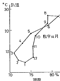
図-2 Climograph (熊本+佐賀) ÷ 2
