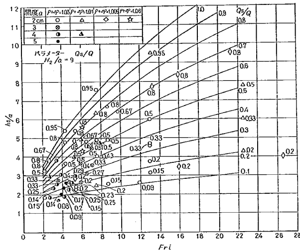
図-5.2 h_s/a \sim F_{ri}
