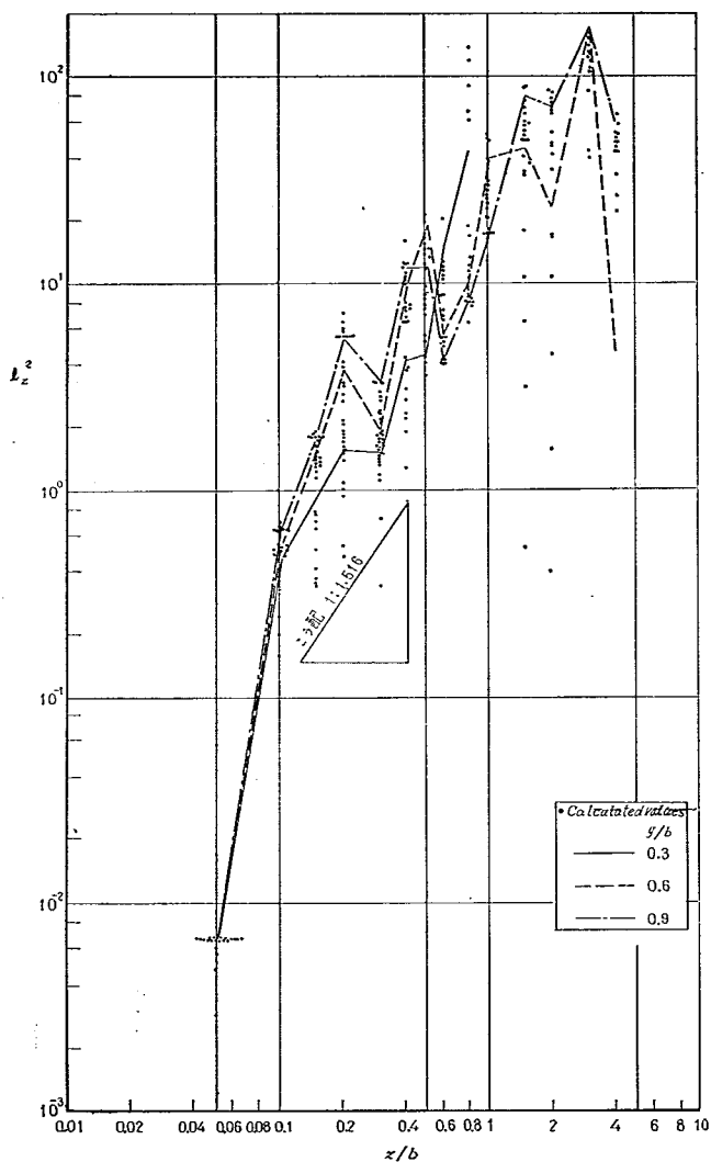
Fig. 9 Mixing length \ell_z Vs. z/b . * Calculated values
