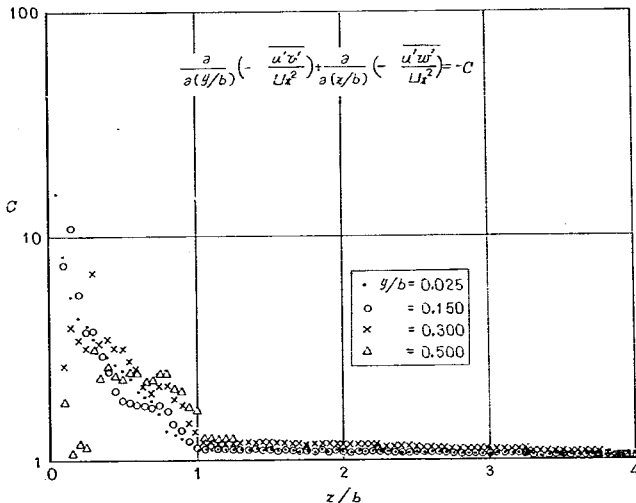
Fig. 3 (a) Verification of constant C
