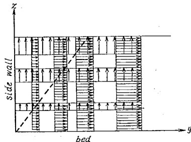
Fig. 16 (b) Profile of shear stress
