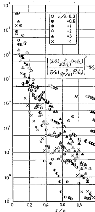
Fig. 11 Ratio of Reynolds stresses Calculated from the measured velocity distribution
