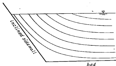
Fig. 21 Velocity distribution near inclined sidewall
