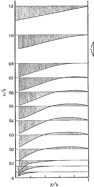
Fig. 12 (a) \overline{u'v'}/u_*^2 distribution (Tracy)
