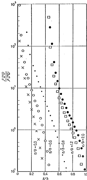
Fig. 10 -\rho \bar{u}'v' / -\rho \bar{u}'w' Vs. y/b . Calculated from Tracy's experiment
