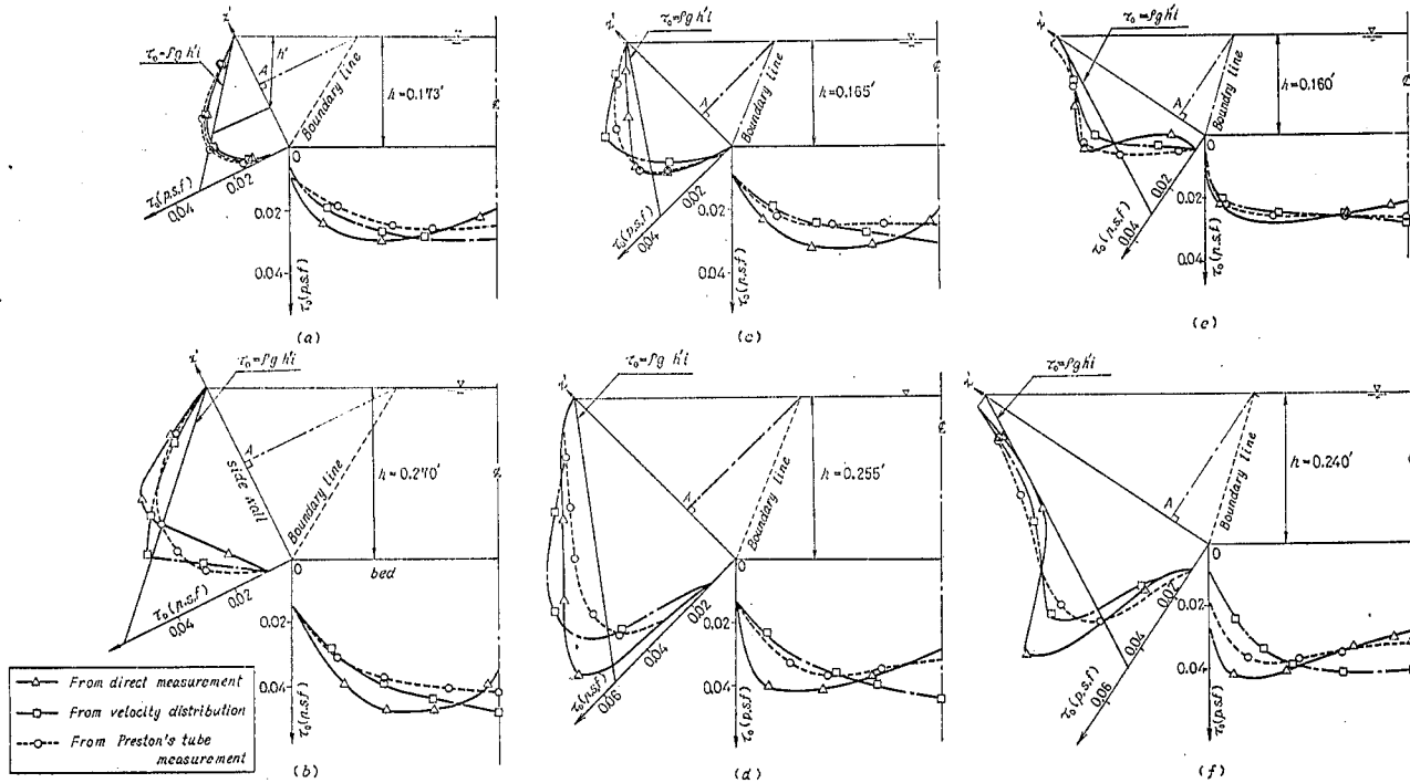
Fig. 23 Boundary shear distribution near inclined sidewall and bed (Ghosh et al) h' : Vertical depth over inclined sidewall
