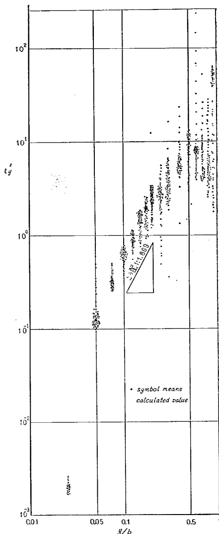
Fig. 8 Mixing Length l_y^2 Vs. y/b . Calculated from Tracy's experiment
