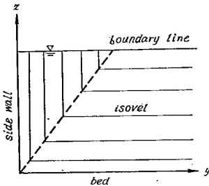
Fig. 15 (a) Profile of isovels
