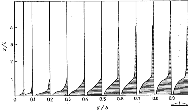
Fig. 12 (b) \overline{u'v'}/u_*^2 distribution (Tracy)
