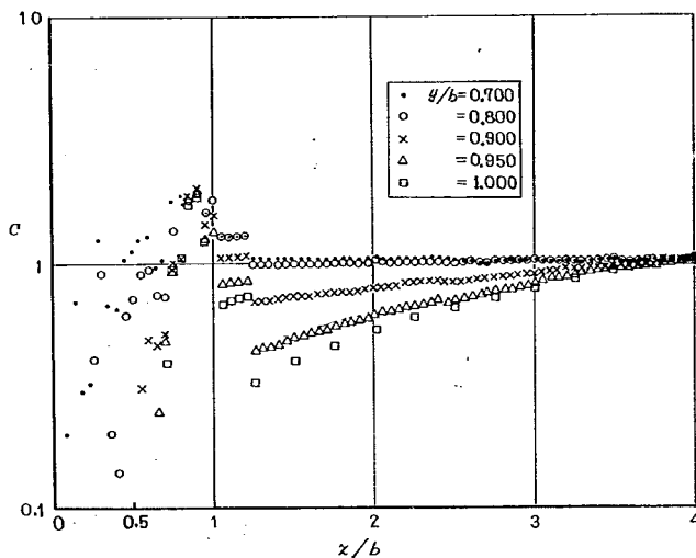
Fig. 3 (b) Verification of constant C
