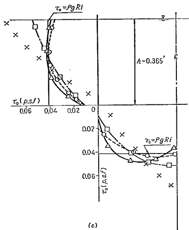
Fig. 20 (e) KC_1 = 8.02 \times 10^{-2} , C_2 = C_3 = 51 \text{ ft}^{-1}
