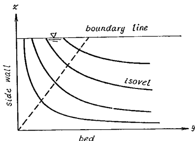
Fig. 16 (a) Profile of isovels
