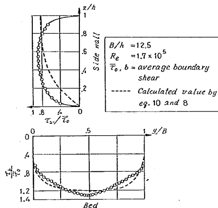
Fig. 19 Boundary shear distribution (Kartha et al)
