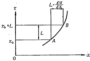
Fig. 5 (b) Mixing length of two-dimensional flow
