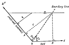
Fig. 22 Boundary line nrofile near inclined sidewall
