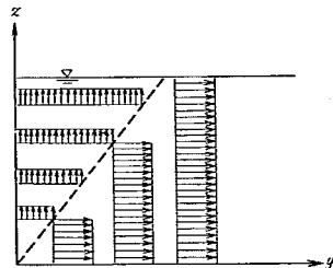
Fig. 15 (b) Profile of shear stress
