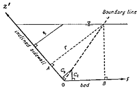
Fig. 22 Boundary line profile near inclined sidewall
