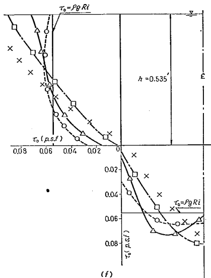
Fig. 20 (f) KC_1 = 8.24 \times 10^{-2} , C_2 = C_3 = 51 \text{ ft}^{-1}
