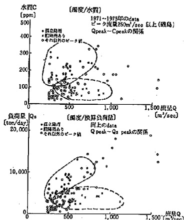
図-25 河川①濁度の Q_{\text{peak}} \sim C_{\text{peak}} (or Q_s peak) の関係
