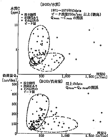
図-26 河川①BODの Q_{\text{peak}} \sim C_{\text{peak}} (or Q_s peak) の関係
