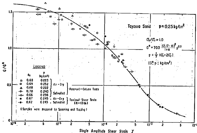
Fig. 4.1 G/G^* versus \gamma relationship of Toyoura Sand ( p = 0.25 kg/cm 2 )
