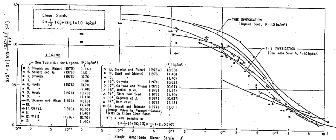
Fig. 5.3 G/G^* versus \gamma relationship of various Clean Sands
