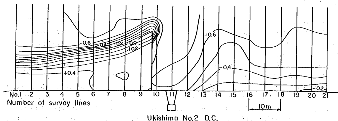
Fig. 11 Beach topography and alignment of survey lines around Ukishima No2 Drainage Channel measured in February, 1985.
