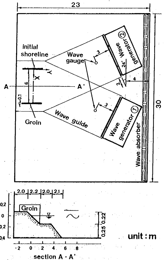
Fig. 15 Experimental set-up of plane wave basin and beach profile.
