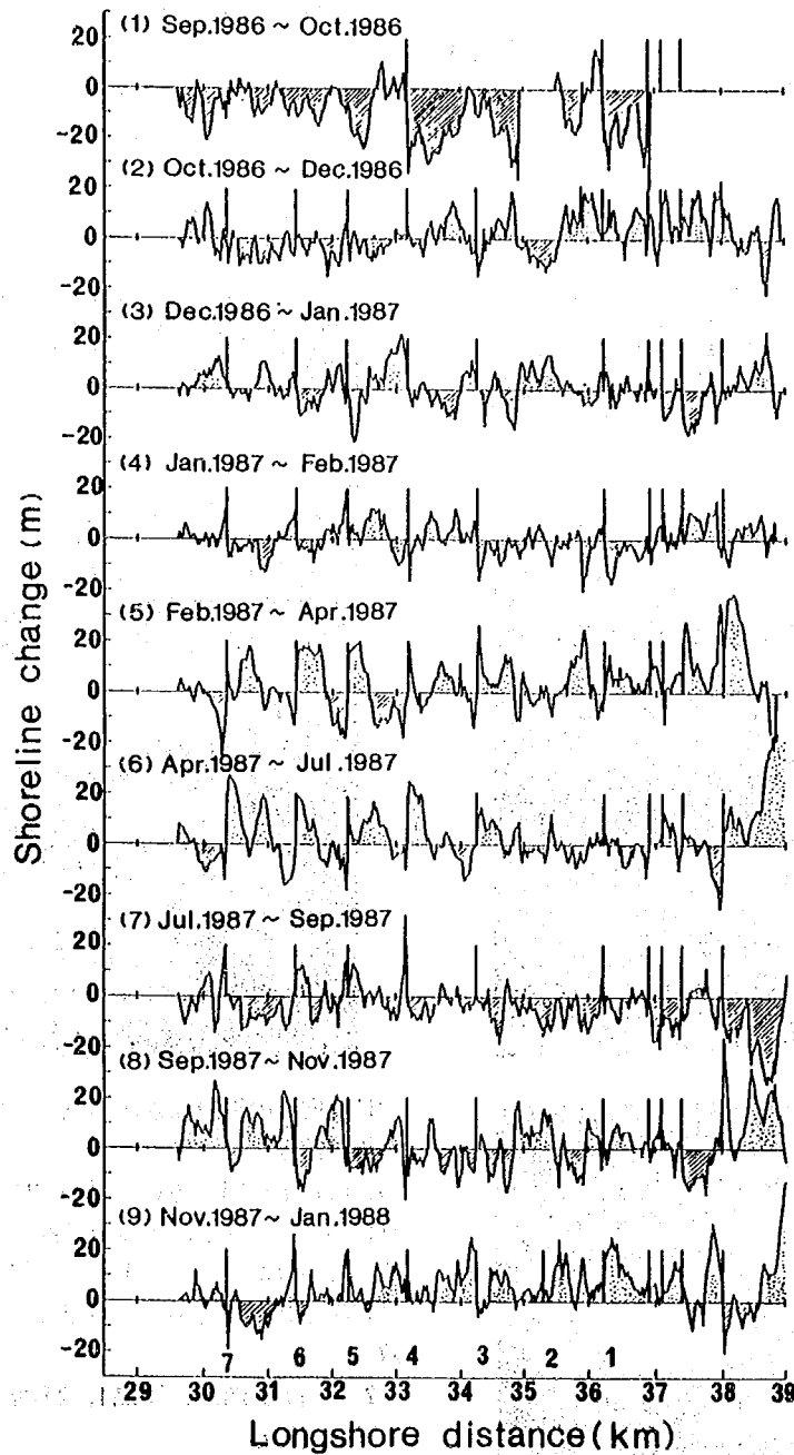
Fig. 4 Spatial and temporal change in shoreline position in the vicinity of headlands on the Kasihmanada Coast between September 1986 and January 1988. These shoreline changes were plotted by the comparison of aerial photographs. Locations of the headlands are shown on the bottom.
