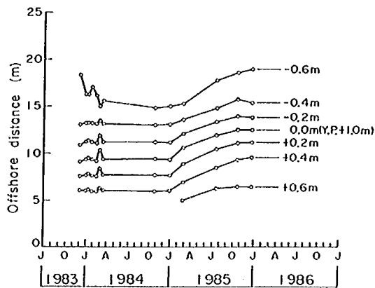
Fig. 7 Temporal change of offshore distances to some contours (Ukishima No.1 Drainage Channel, Survey line No.1).
