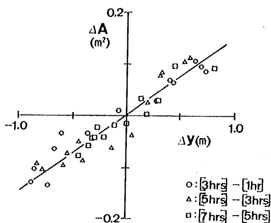
Fig. 24 Relationship between the change of the cross-sectional area ( \Delta A ) and the shoreline change ( \Delta y ).
