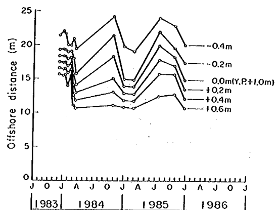
Fig. 10 Temporal change of offshore distances to some contours (Ukishima No1 Drainage Channel, Survey line No18).
