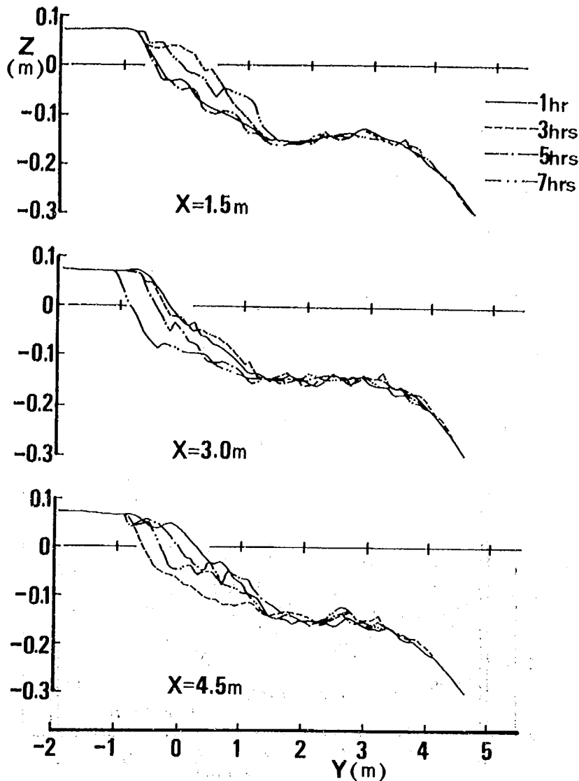
Fig. 20 Change in beach profiles at three sections.
