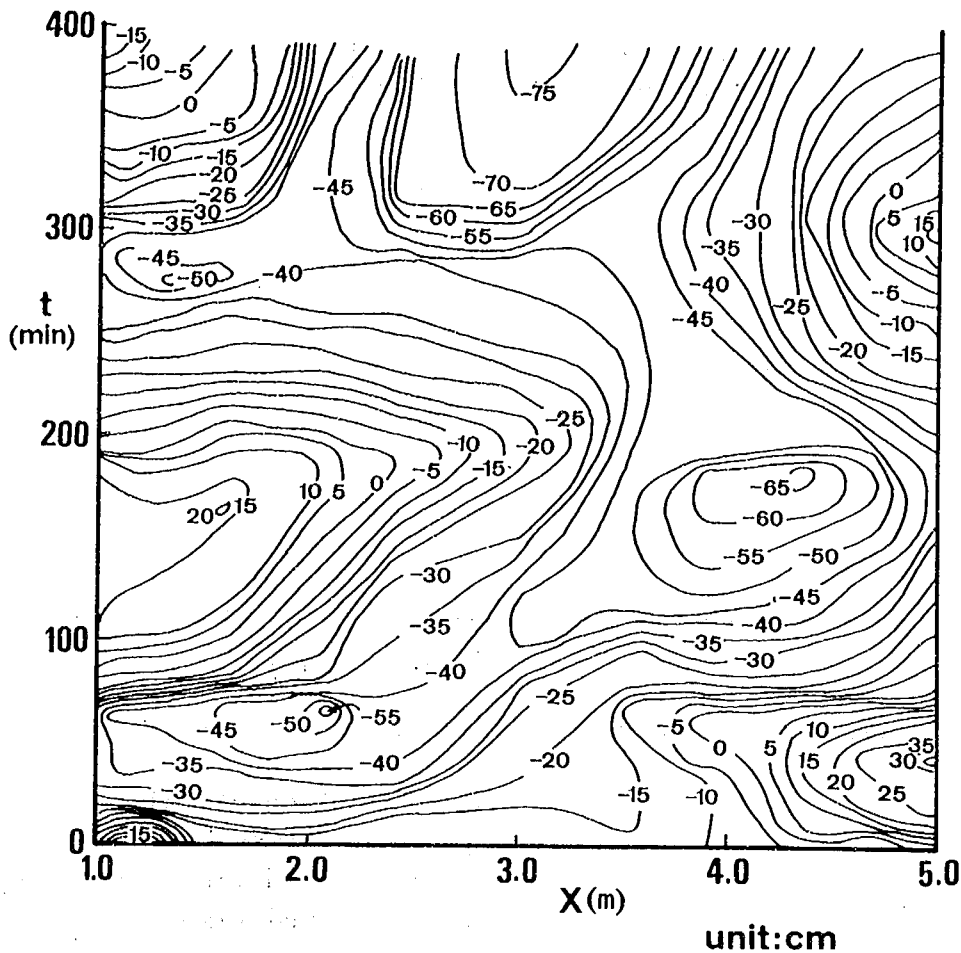
Fig. 26 Temporal change of shoreline position (Experimental result).
