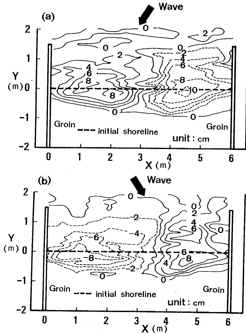
Fig. 21 Distribution of contours connecting equal change in depth.
