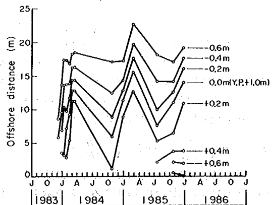
Fig. 14 Temporal change of offshore distances to some contours (Ukishima No2 Drainage Channel, Survey line No9).
