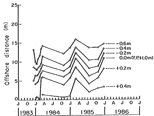
Fig. 13 Temporal change of offshore distances to some contours (Ukishima No2 Drainage Channel, Survey line No5).
