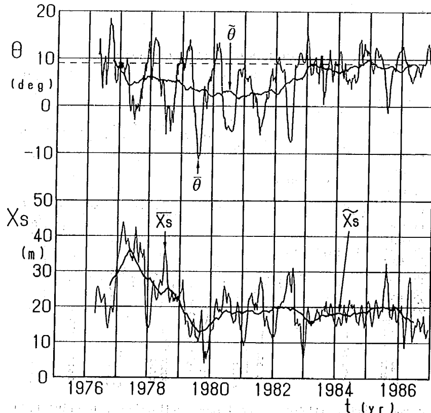
Fig. 3 Long-term changes of wave direction ( \theta ) and shoreline position ( X_s ) at Ajigaura Beach.
