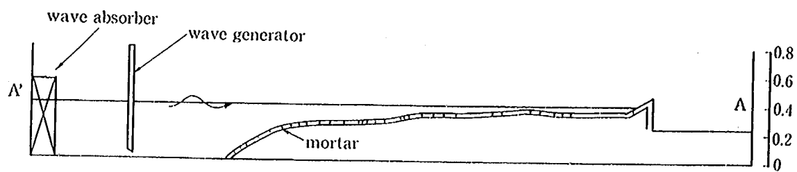
Profile of A-A' section
