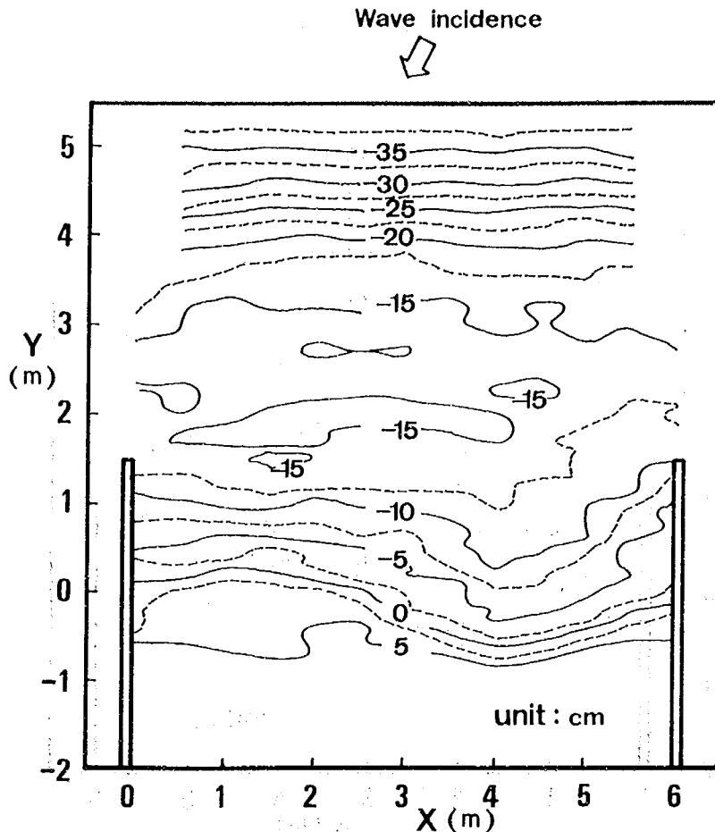
Fig. 18 Contours measured at 3 hours from the beginning.
