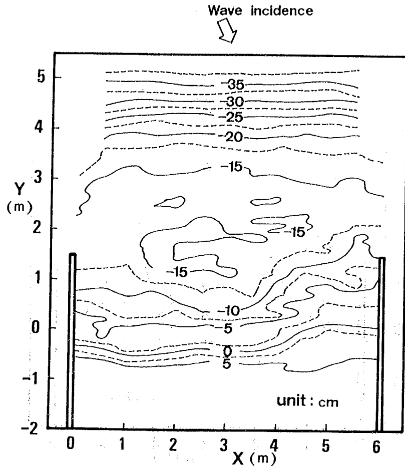
Fig. 19 Contours measured at 5 hours from the beginning.
