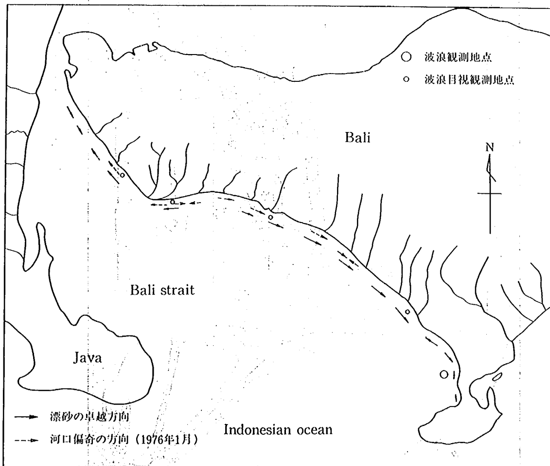
図-2.7 バリ海峡沿岸の漂砂の卓越方向 (Tsuchiya, 1975)
