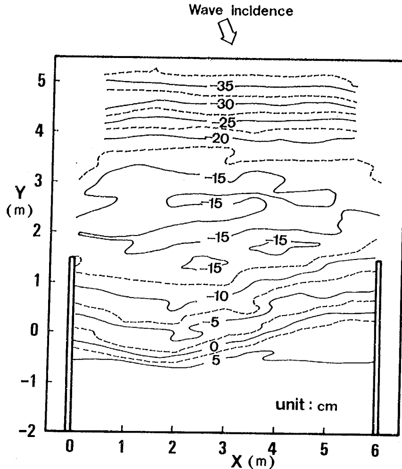
Fig. 17 Contours measured at 1 hour from the beginning.
