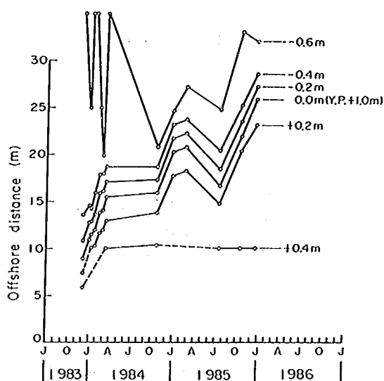
Fig. 9 Temporal change of offshore distances to some contours (Ukishima No1 Drainage Channel, Survey line No9).
