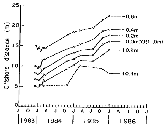
Fig. 8 Temporal change of offshore distances to some contours (Ukishima No.1 Drainage Channel, Survey line No.5).
