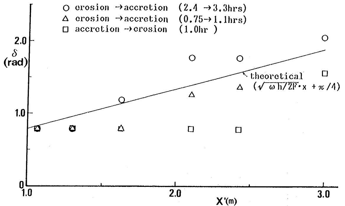
Fig. 27 Comparison of phase difference between wave direction and shoreline position.
