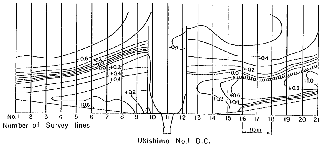
Fig. 6 Beach topography and alignment of survey lines around Ukishima No.1 Drainage Channel measured in February, 1985.
