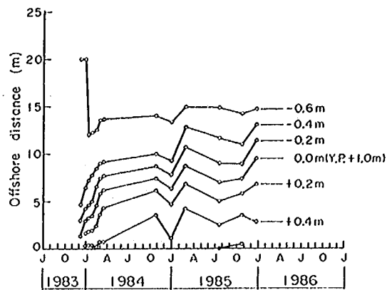
Fig. 12 Temporal change of offshore distances to some contours (Ukishima No2 Drainage Channel, Survey line No1).
