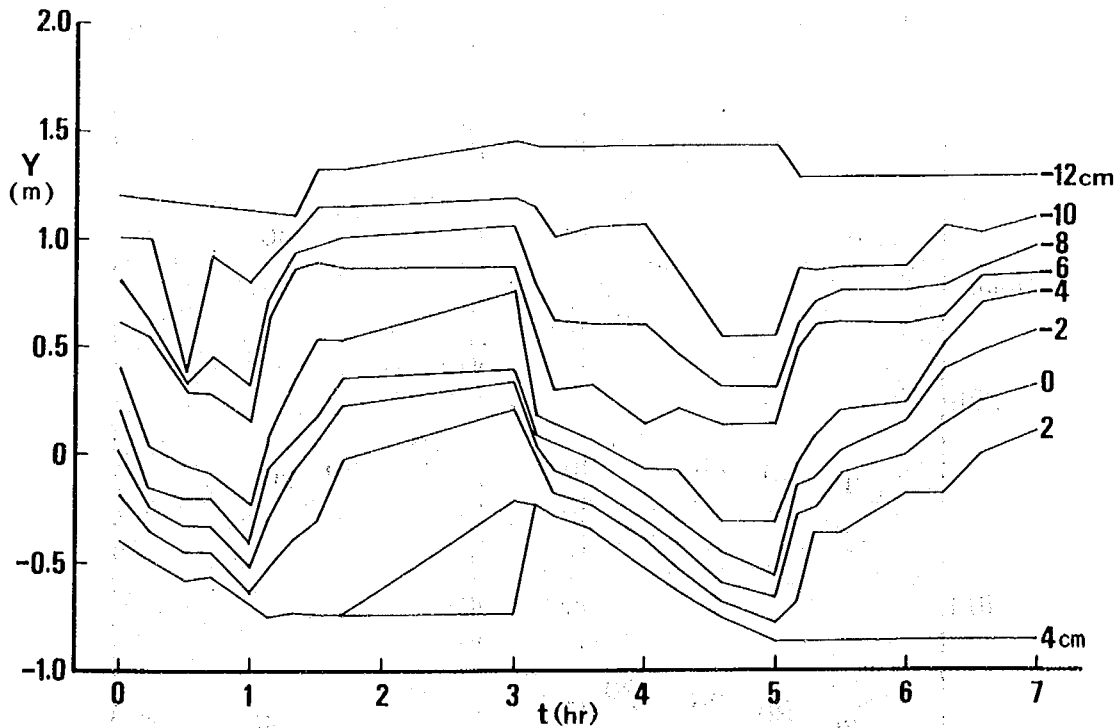
Fig. 23 Temporal change in offshore distances at a section of X = 1.0\text{m} .
