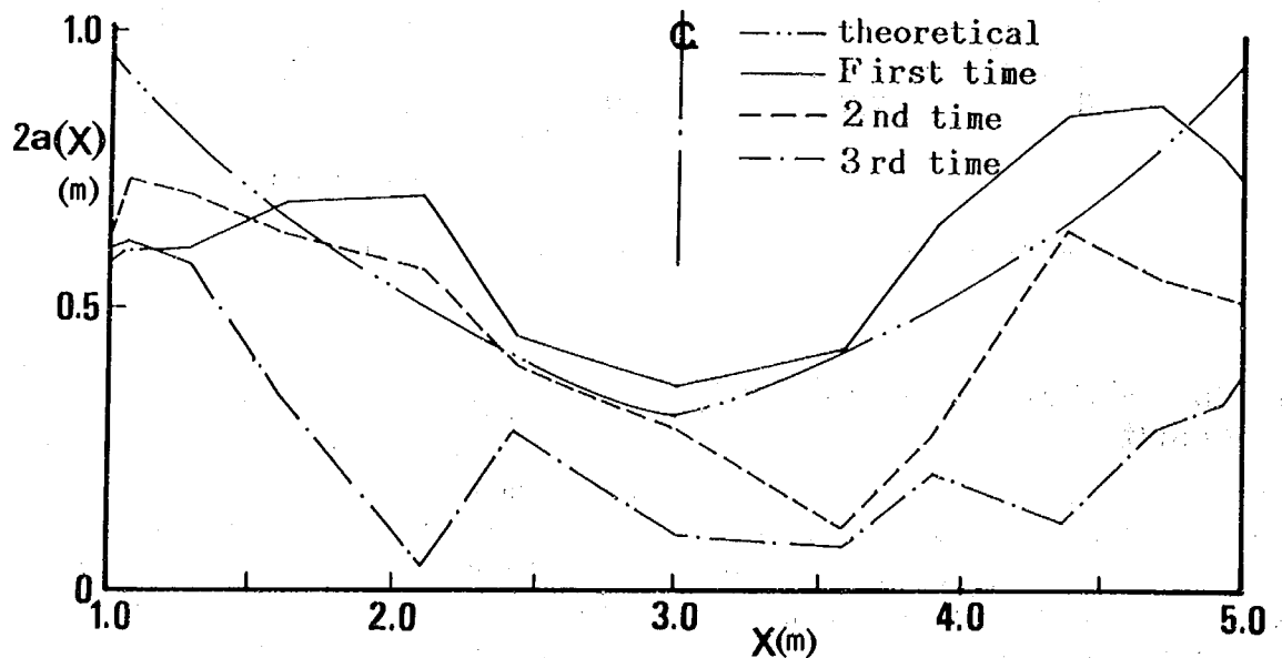
Fig. 28 Comparison of amplitude of shoreline change.
