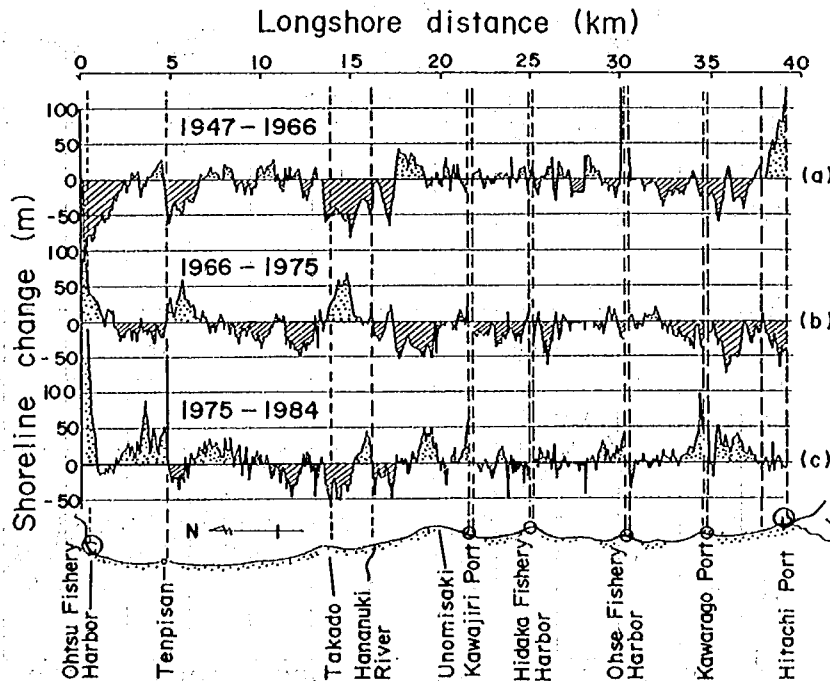
Fig. 2 Shoreline changes between Ohtsu Fishery Harbor and Hitachi Port from 1947 to 1984. These changes were plotted by the comparison of aerial photographs.
