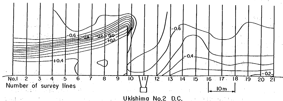
Fig. 11 Beach topography and alignment of survey lines around Ukishima No2 Drainage Channel measured in February, 1985.
