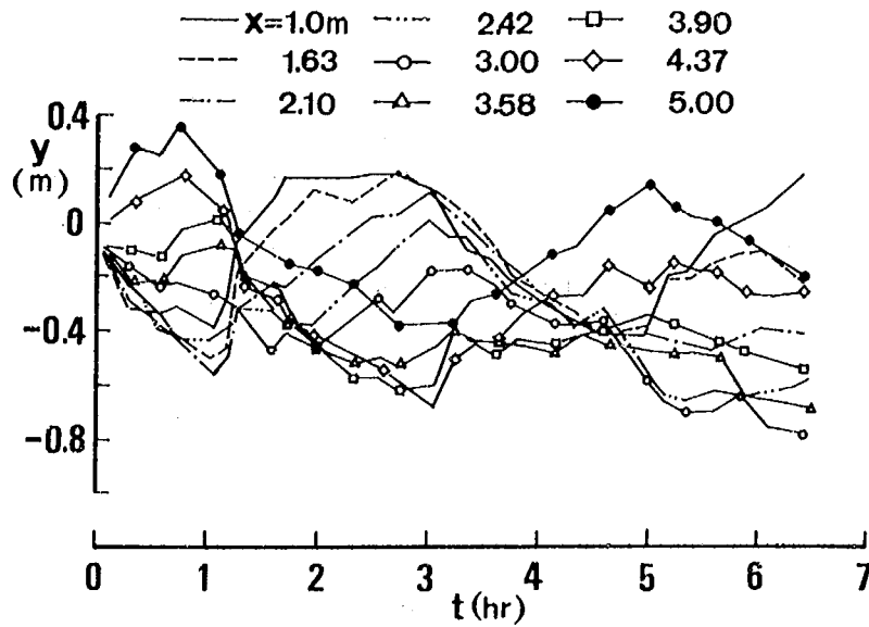
Fig. 22 Temporal changes in shoreline position.
