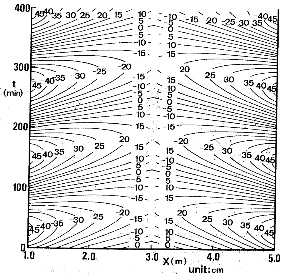
Fig. 25 Temporal change of shoreline position (Theoretical solution).
