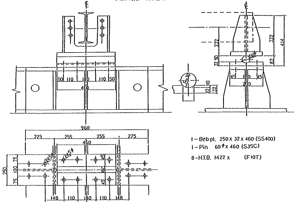
図-1.3.4 (b) 支点治具の寸法形状
