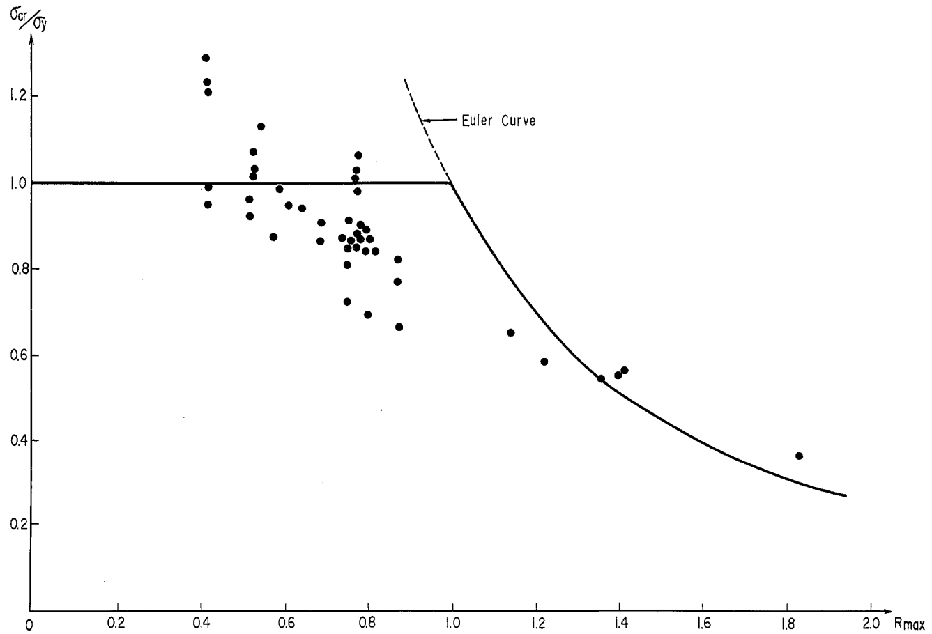
Fig. 2.4 ULTIMATE STRENGTH
