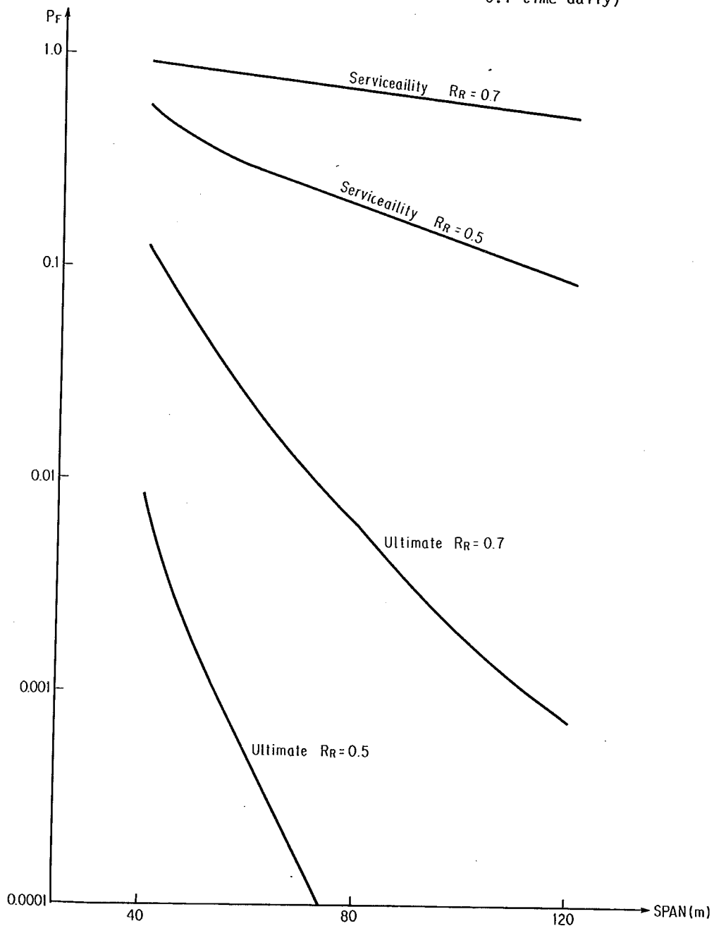
Fig. 4.2 PROBABILITY OF FAILURE OF BOX GIRDER BRIDGES
