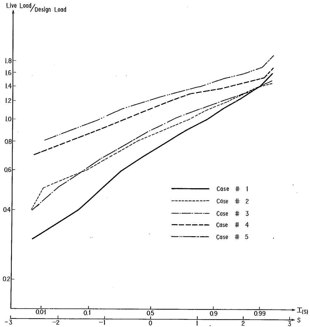
Fig. 3.4(b) SIMULATED LIVE LOAD (SPAN = 80m) (on lognormal probability paper)
