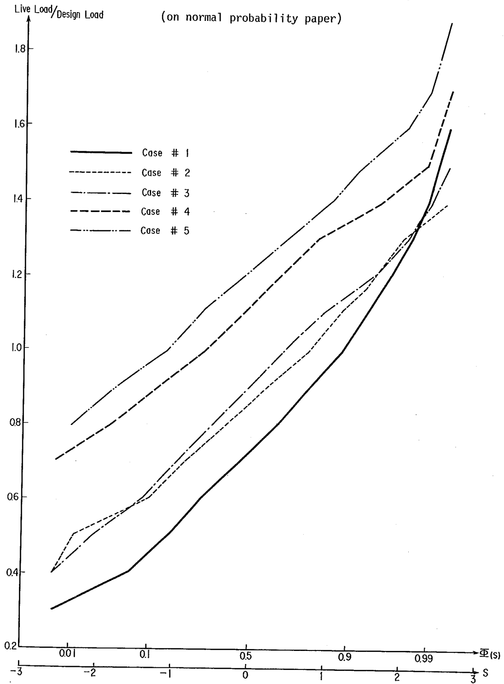
Fig. 3.4(a) SIMULATED LIVE LOAD (SPAN = 80m)
