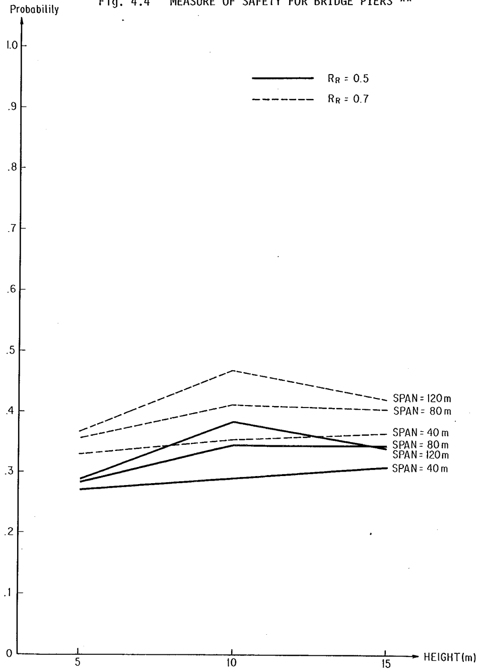
Fig. 4.4 MEASURE OF SAFETY FOR BRIDGE PIERS **
