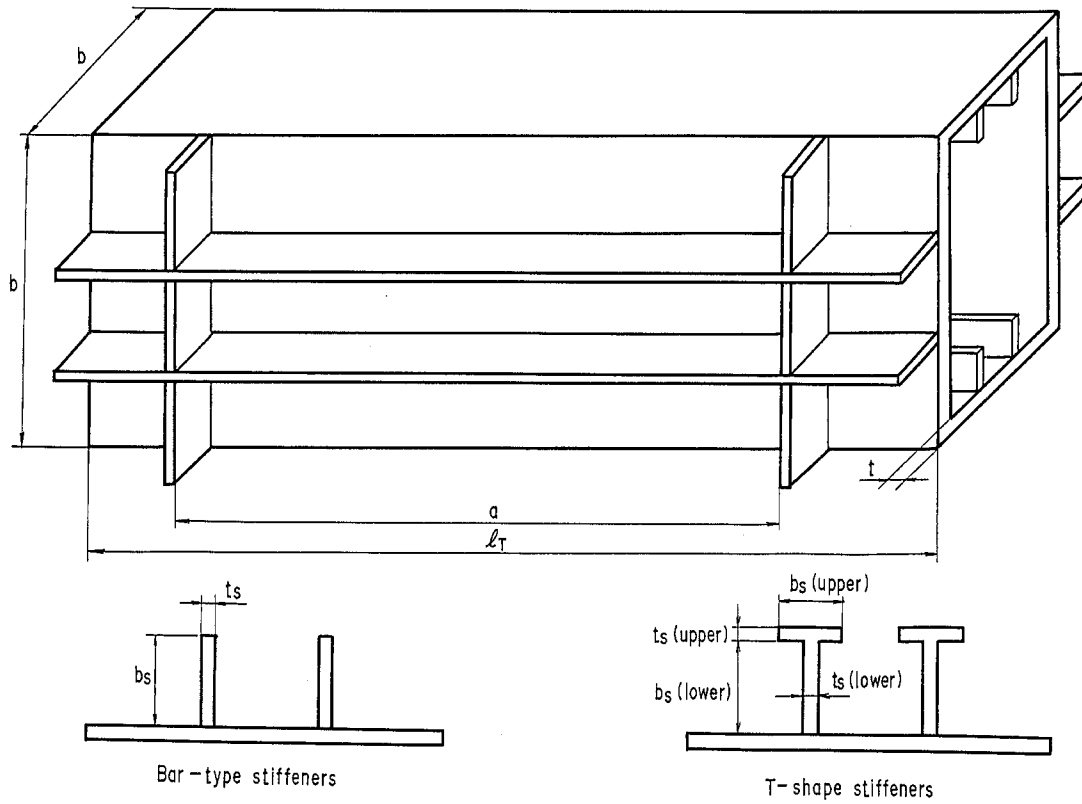
Fig. 2.1 TYPICAL CONFIGURATION OF TEST SPECIMENS
