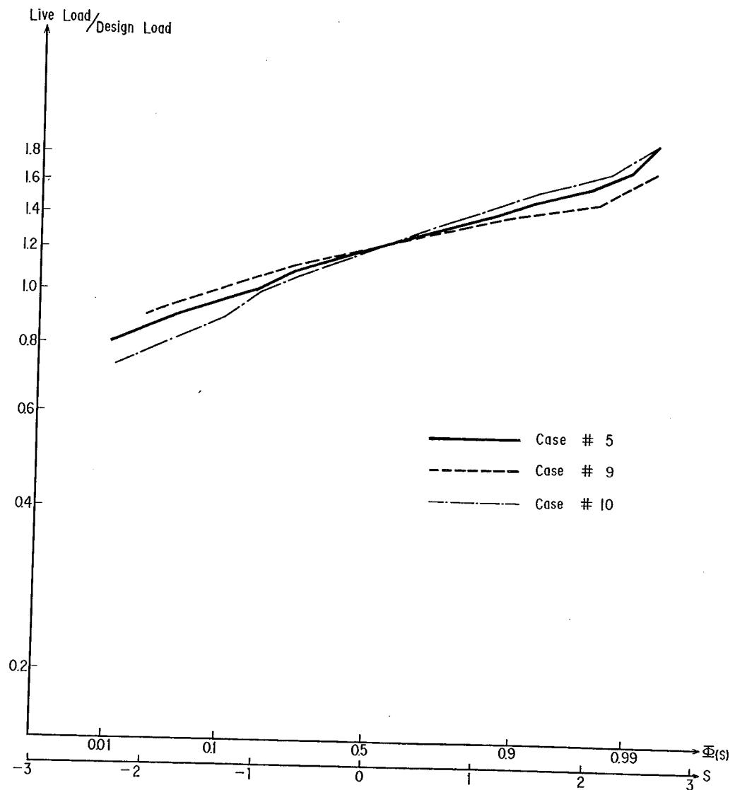
Fig. 3.6 EFFECT OF C.O.V. ON SIMULATED LIVE LOAD (on lognormal probability paper)
