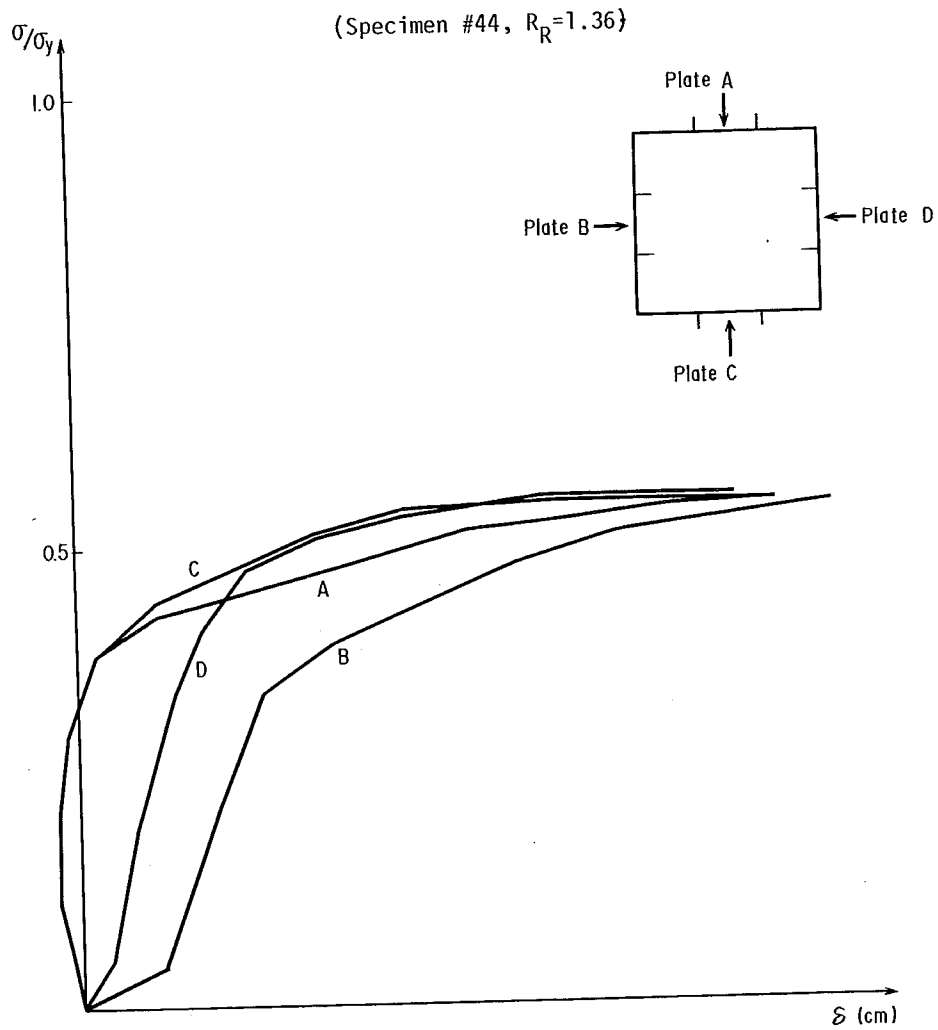
Fig. 2.5 OUT-OF-PLANE DEFLECTION
