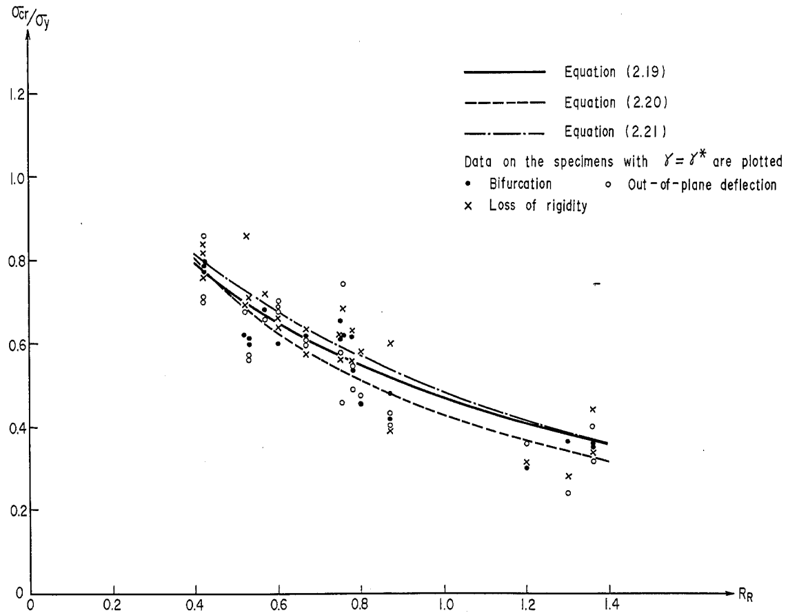
Fig. 2.7(b) SERVICEABILITY LIMITS ( \gamma=\gamma^* )
