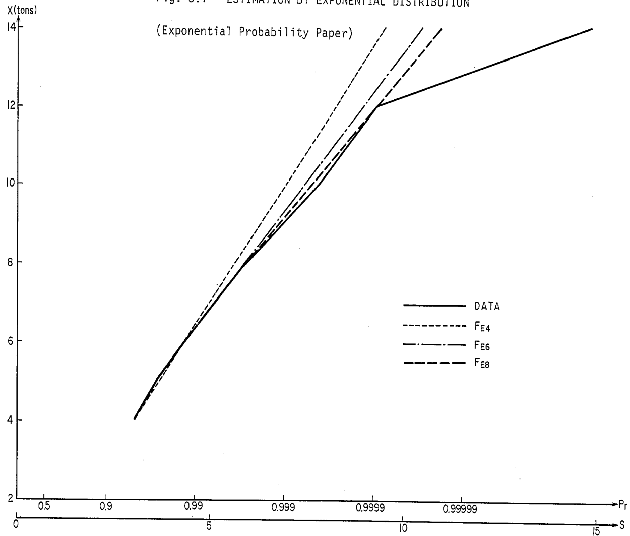
Fig. 3.1 ESTIMATION BY EXPONENTIAL DISTRIBUTION
