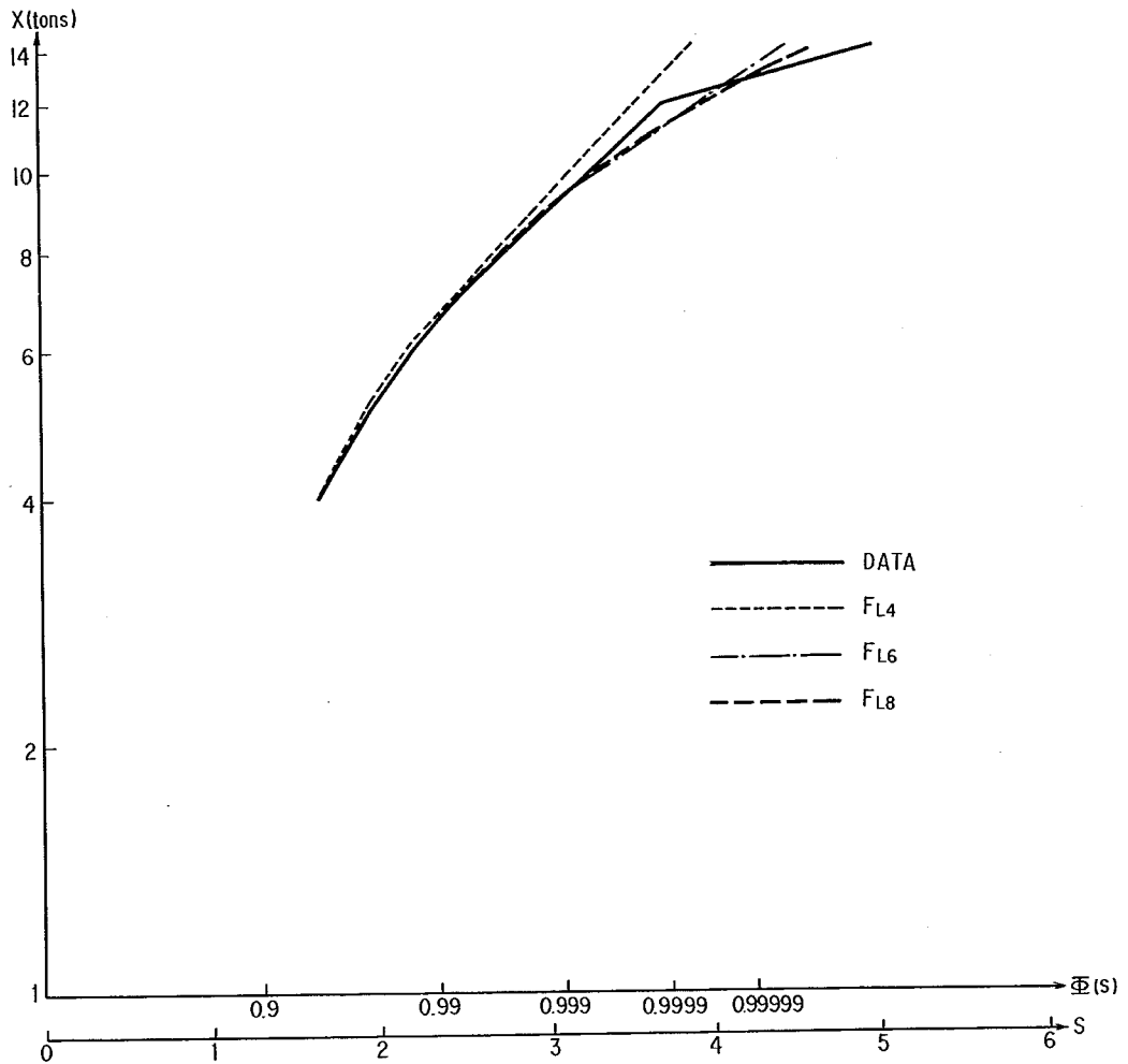
Fig. 3.3 ESTIMATION BY LOGNORMAL TAIL
