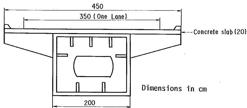
Fig. 4.1 CROSS SECTION OF TYPICAL BOX GIRDER BRIDGE
