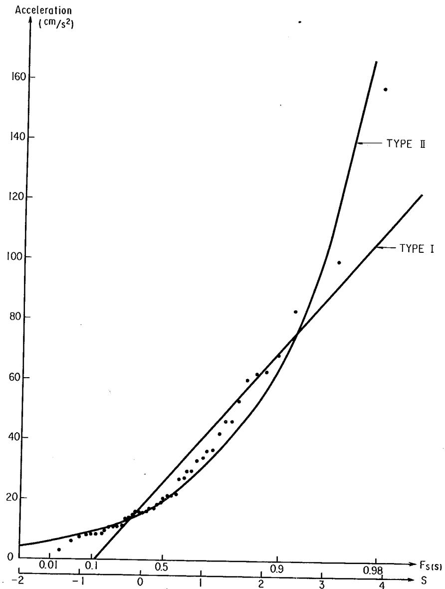
Fig. 3.7 PLOTS ON GUMBEL PROBABILITY PAPER (annual maximum acceleration)
