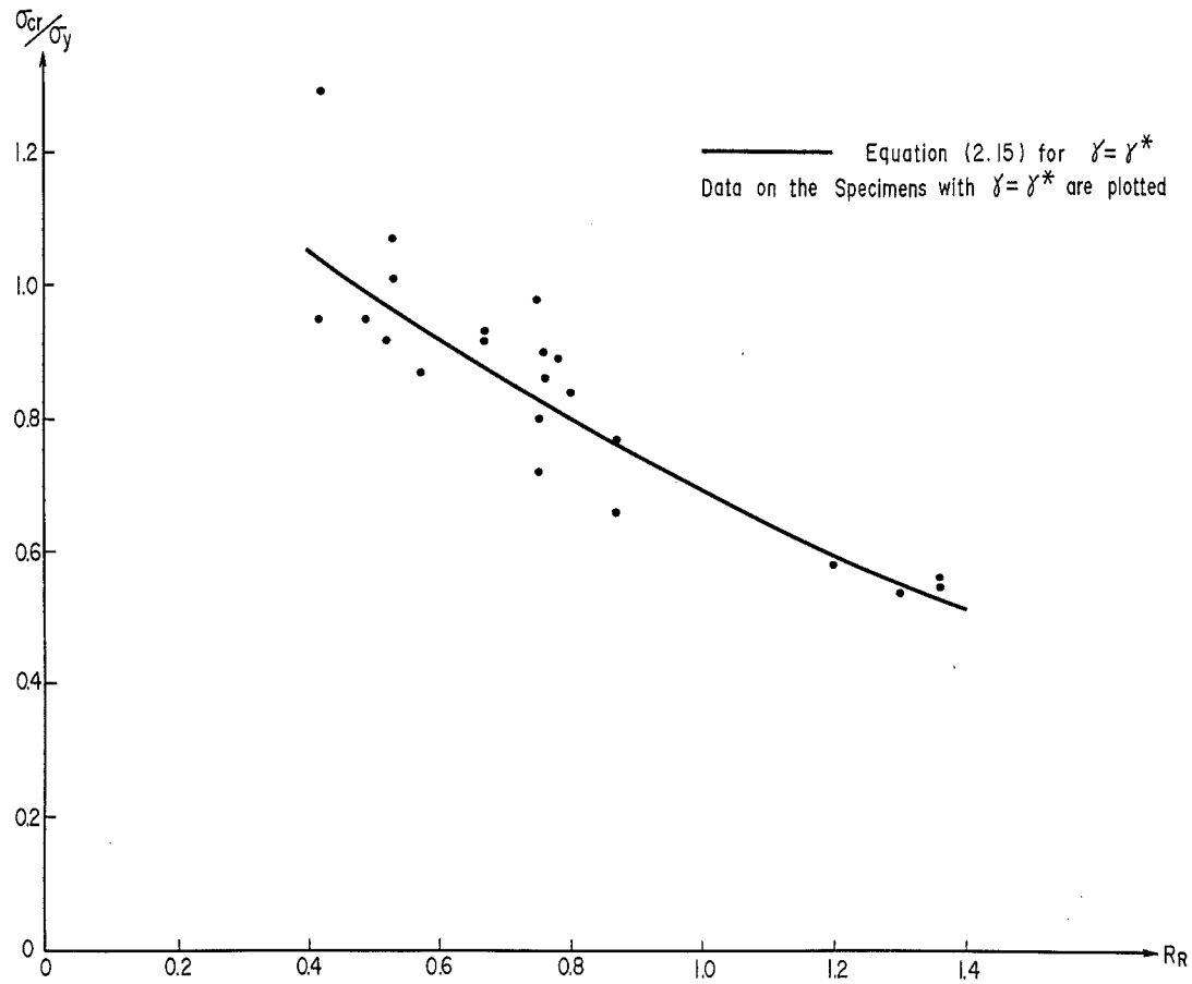
Fig. 2.7(a) ULTIMATE STRENGTH ( \gamma=\gamma^* )
