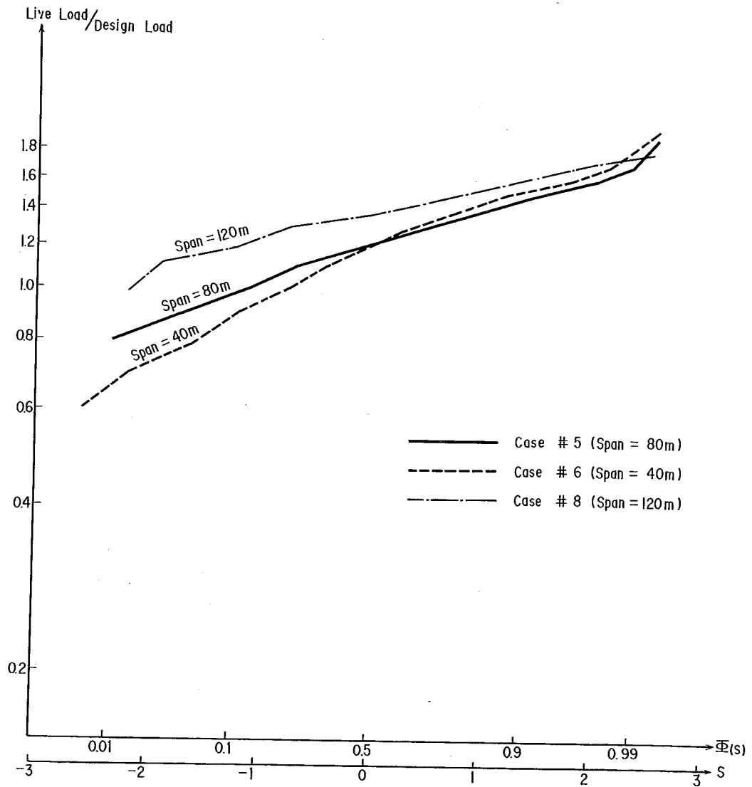
Fig. 3.5 SIMULATED LIVE LOAD FOR VARIOUS SPAN LENGTHS (on lognormal probability paper)
