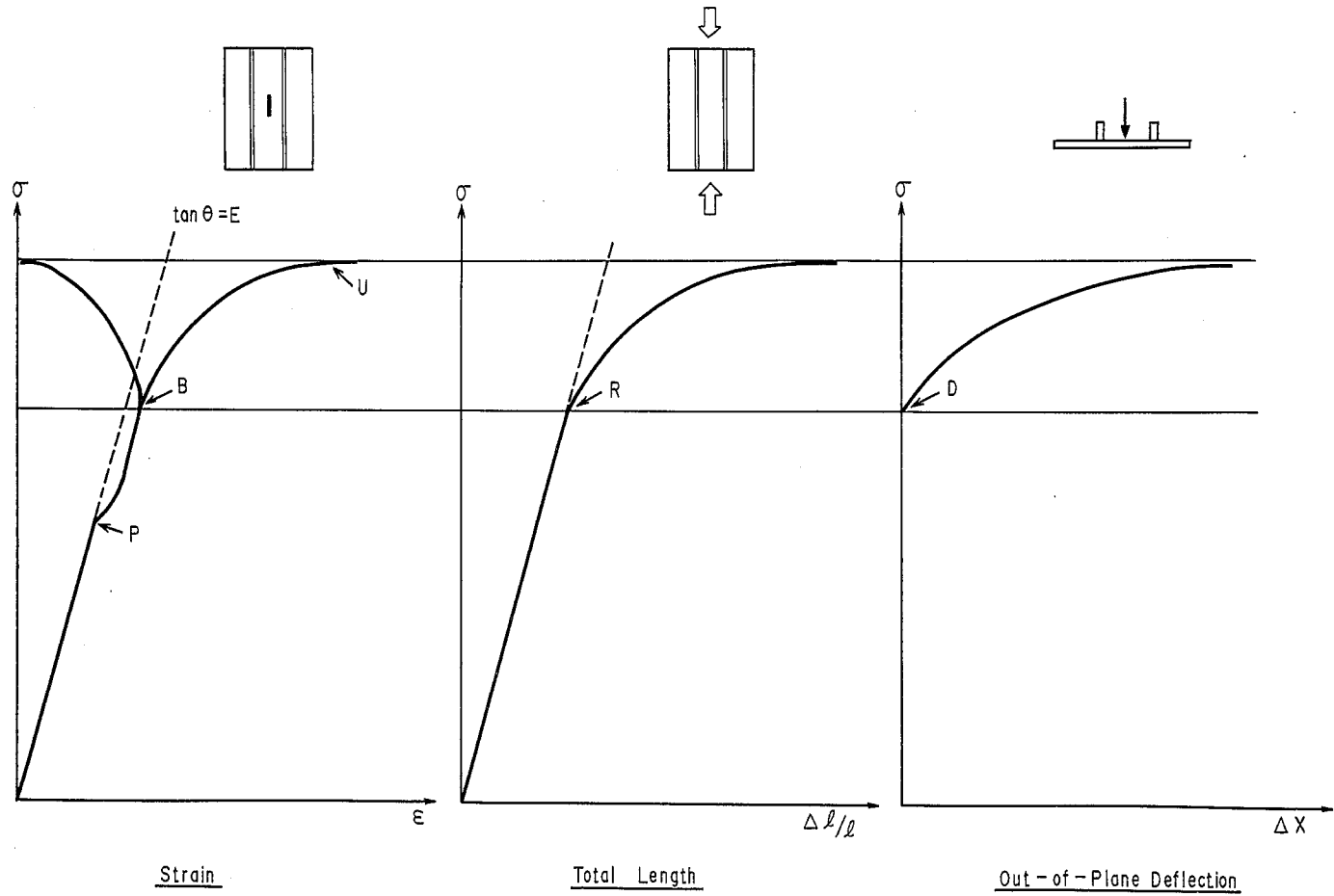
Fig. 2.3 LIMIT STATES
