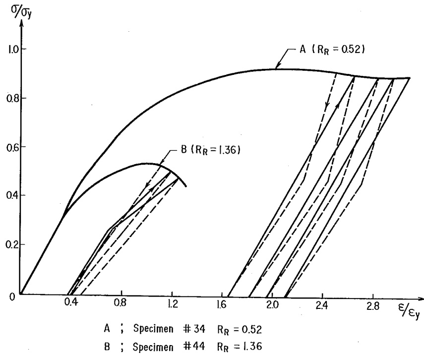
Fig. 2.6 RESISTANCE TO REPEATED LOAD
