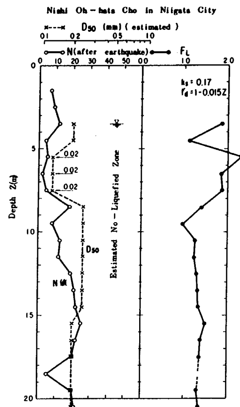
Fig. 2 Relationships between F_L and Z at the Non-Liquefied Site
