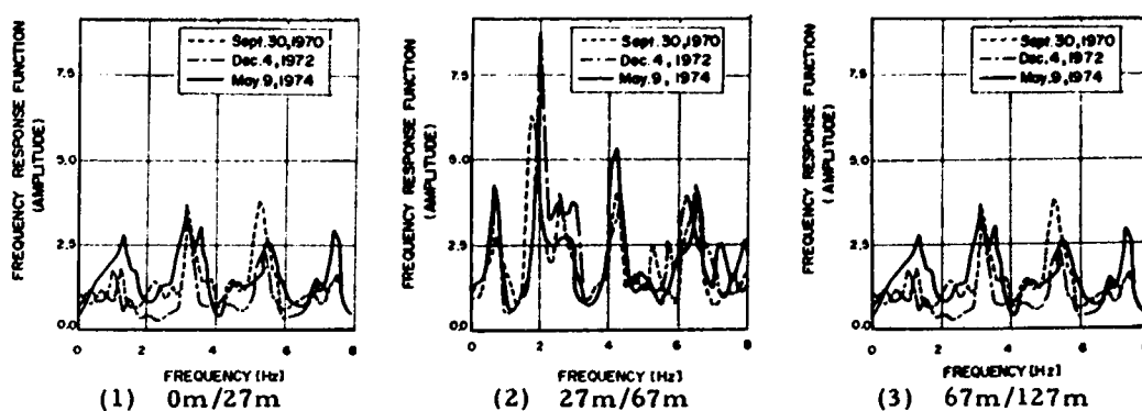
FIG. 3 FREQUENCY RESPONSE FUNCTION (AMPLITUDE) BETWEEN TWO ADJACENT RECORDING POINTS (UKISHIMA PARK, HORIZONTAL COMPONENT)
