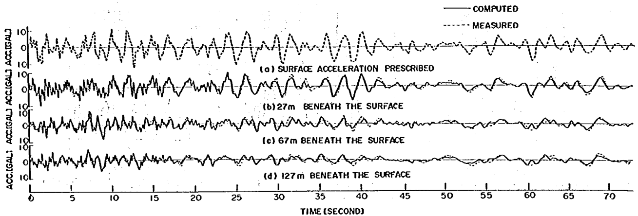
FIG. 6 CORRELATION OF COMPUTED AND MEASURED UNDERGROUND ACCELERATION (UKISHIMA PARK, NS COMPONENT)
