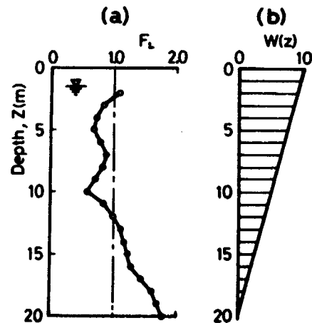
Fig. 1 Integration of F_L
