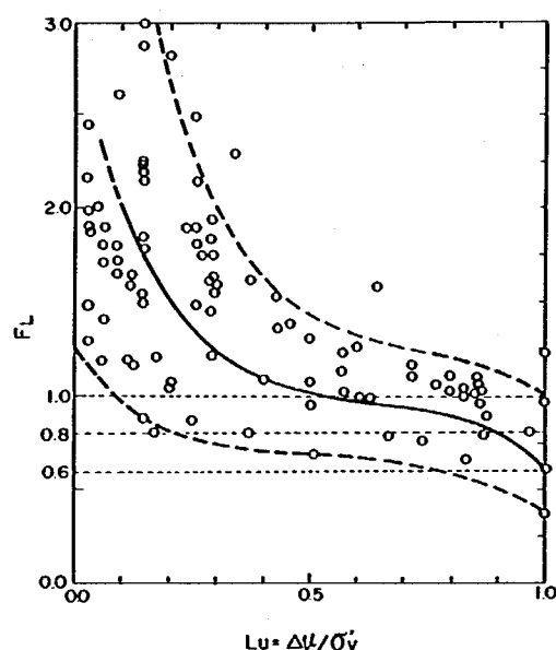
Fig. 10 Relationships between F_L Values and the Rate of Ground Liquefaction \Delta u/\sigma_v' in Shaking Table Tests
