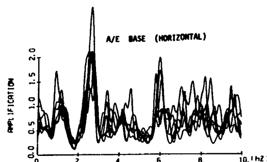
Fig. 34 FRF (Amplification) of A67 to E50 in Horizontal (Tsuchida et al (1978))
