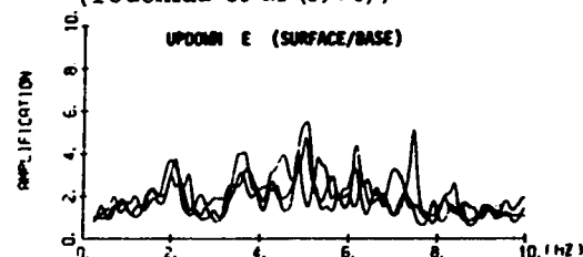
Fig. 33 FRF (Amplification) of E to E50 in Vertical (Tsuchida et al (1978))
