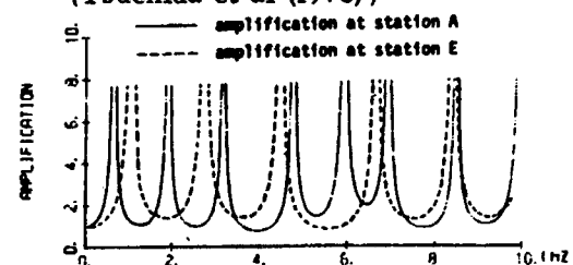
Fig. 36 FRF (Amplification) of Multiple Reflection Model with No Damping (Tsuchida et al (1978))
