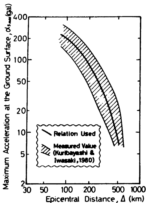
Fig. 4 Relation between Maximum Acceleration at the ground surface, \alpha_{smax} , and Epicentral Distance, \Delta , during the Miyagi-ken-oki Earthquake
