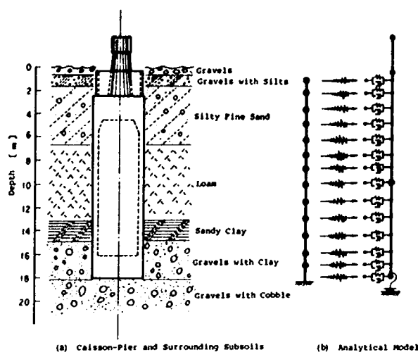
Fig. 68 Analytical Model of Foundation of the Itajima Bridge
