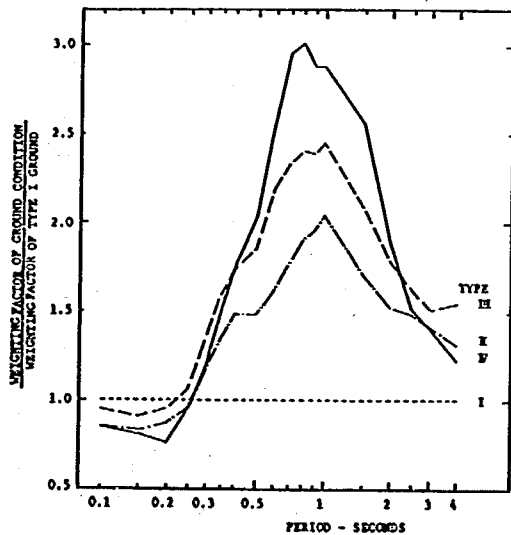
Fig. 14 Effect of Soil Condition on Acceleration Spectra (Katayama et al (1977))
