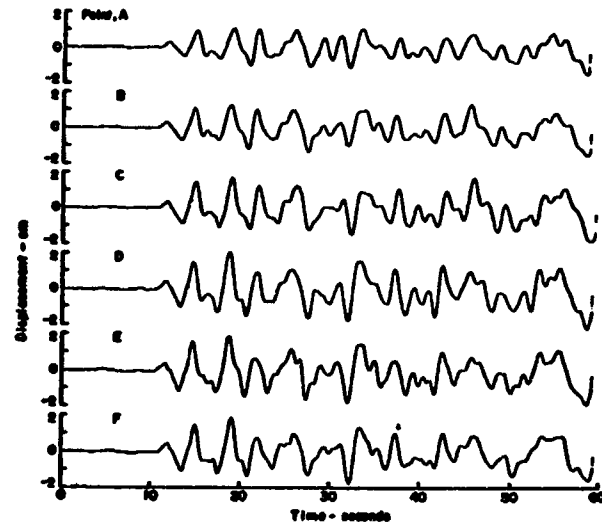
Fig. 26 Calculated Ground Displacements (TIA-3, Longitudinal Component) (Tsuchida et al (1977))
