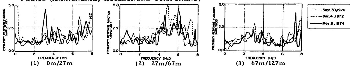
FIG. 5 FREQUENCY RESPONSE FUNCTION (AMPLITUDE) BETWEEN TWO ADJACENT RECORDING POINTS (UKISHIMA PARK, VERTICAL COMPONENT)
