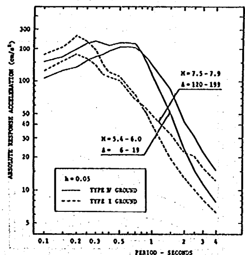
Fig. 11 Example of Predicted Acceleration Spectra (Katayama et al (1977))
