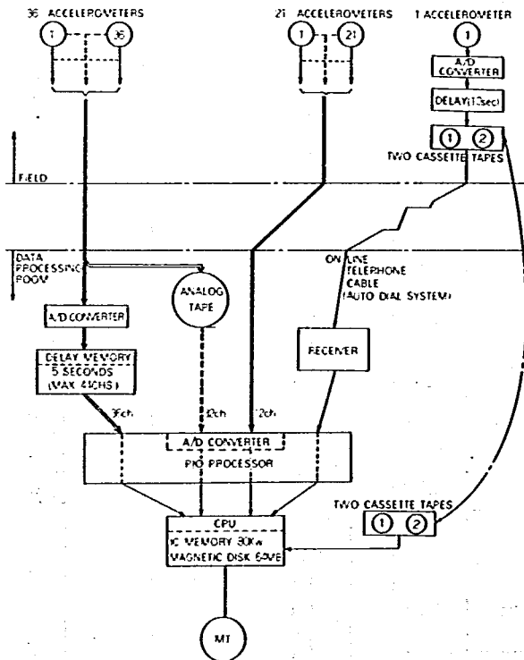
Fig. 46 Data Processing System
