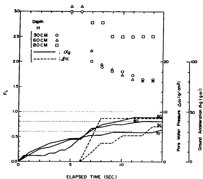
Fig. 8 Relationships between Pore Water Pressure and Acceleration of Non-Liquefied Sand Layers and F_L Values in Shaking Table Tests
