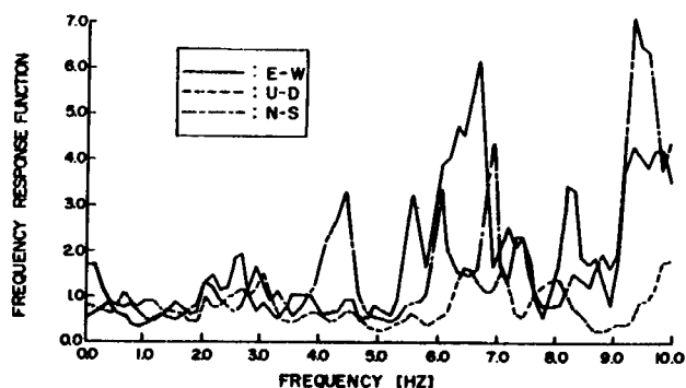
Fig. 64 Frequency Response Function of Station 5 to Station 1, for 3 Components
