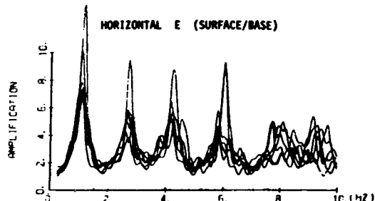
Fig. 31 FRF (Amplification) of E to E50 in Horizontal (Tsuchida et al (1978))
