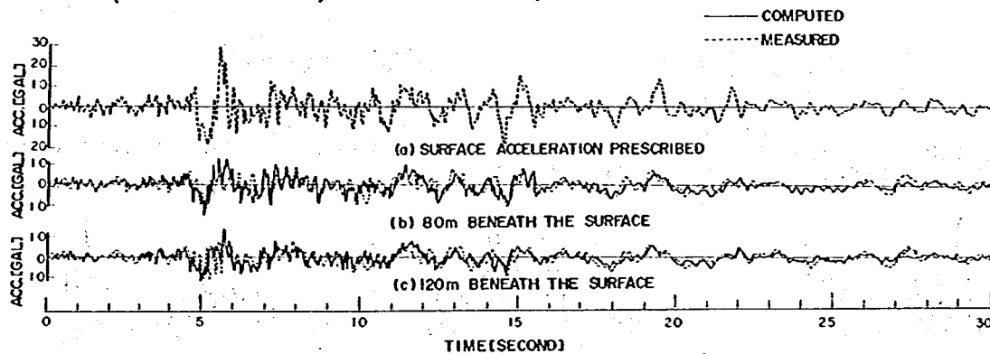
FIG. 7 CORRELATION OF COMPUTED AND MEASURED UNDERGROUND ACCELERATION (KANNONZAKI, NS COMPONENT)
