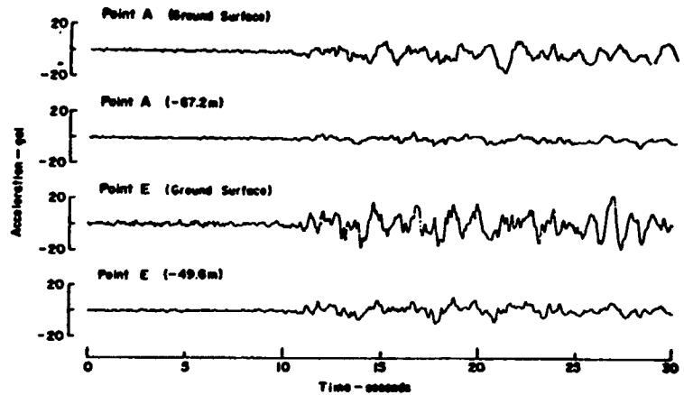
Fig. 25 Observed Ground Accelerations (TIA-3, Longitudinal Component) (Tsuchida et al (1977))
