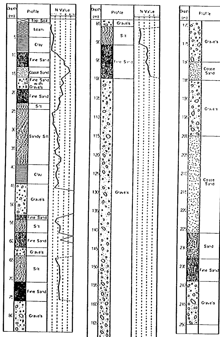
Fig. 45 Soil Profile at PWR1 in Tsukuba Science City
