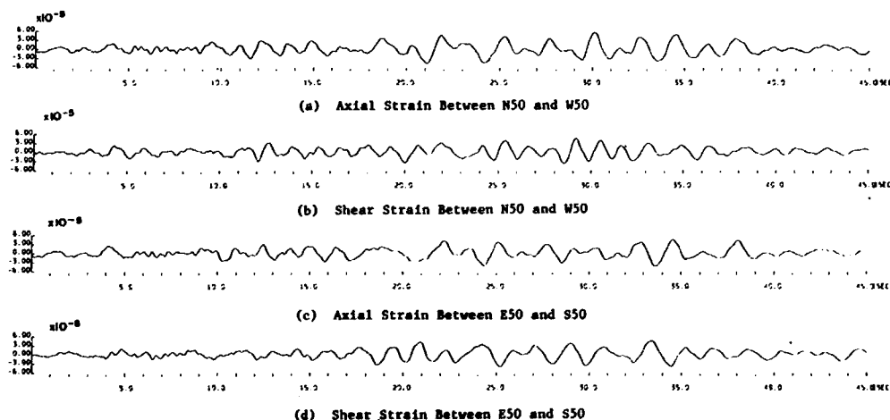
Fig. 52 Axial and Shear Strains Between Two Points
