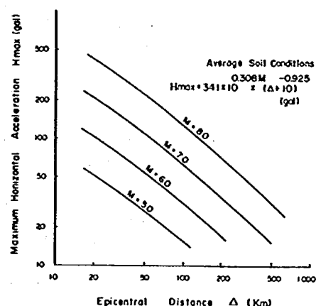
Fig. 3 Example of Epicentral Distance vs. Peak Horizontal Acceleration
