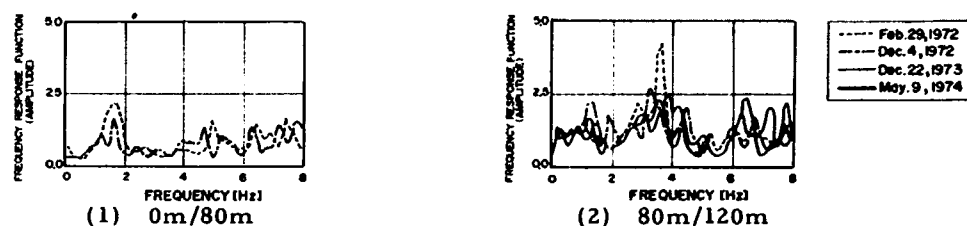
FIG. 4 FREQUENCY RESPONSE FUNCTION (AMPLITUDE) BETWEEN TWO ADJACENT RECORDING POINTS (KANNONZAKI, HORIZONTAL COMPONENT)
