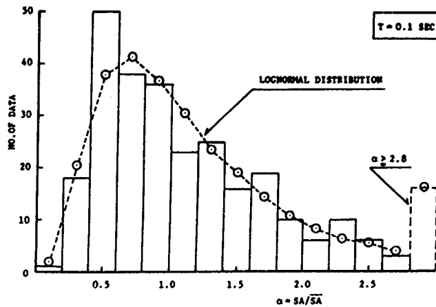
Fig. 16 Histogram of \alpha for T=0.1 sec
