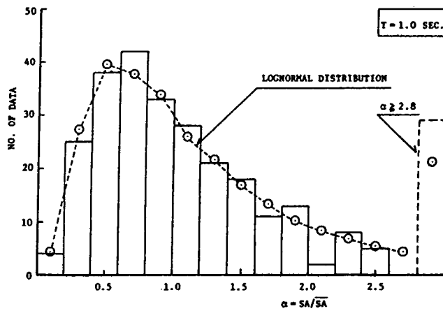
Fig. 18 Histogram of \alpha for T=1.0 sec
