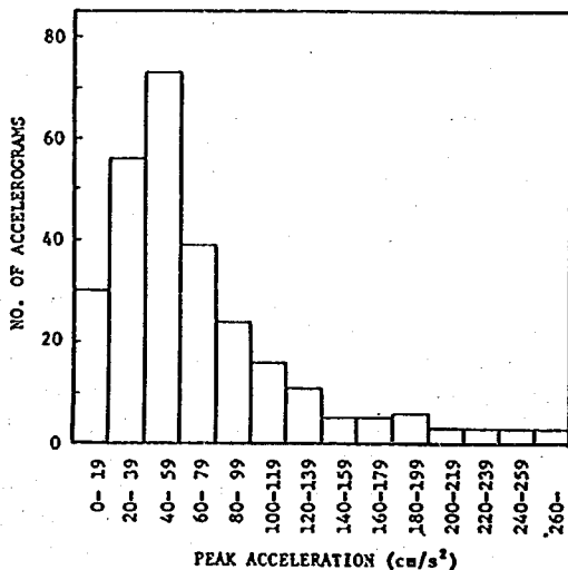
Fig. 10 Histogram of Peak Acceleration of 277 Accelerograms Used for Analysis (Katayama et al (1977))
