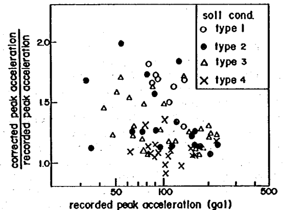
Fig. 5 Amplification of Peak Acceleration due to Correction (Goto et al (1978))
