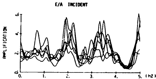
Fig. 37 FRF (Amplification) between E and A (Calculated Incident Waves) (Tsuchida et al (1978))
