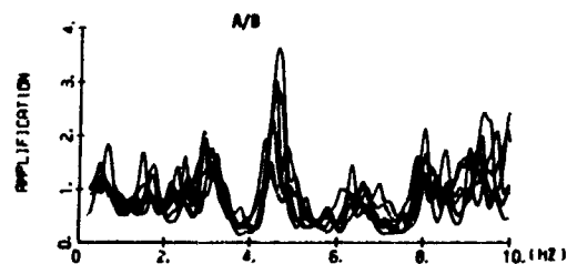
Fig. 27 FRF (Amplification) of A to B (Tsuchida et al (1978))
