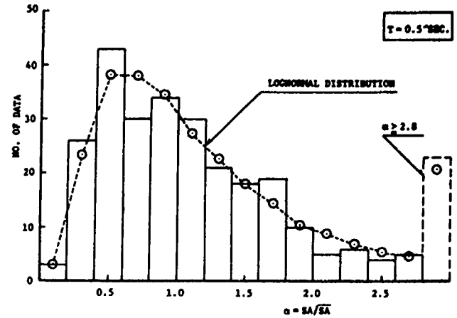
Fig. 17 Histogram of \alpha for T=0.5 sec
