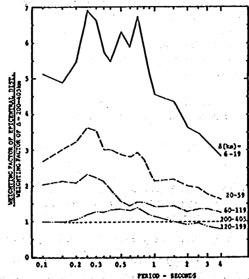
Fig. 13 Effects of Epicentral Distance on Acceleration Spectra (Katayama et al (1977))
