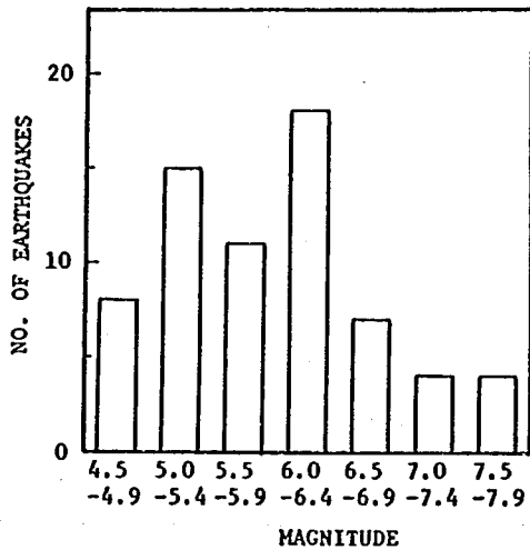
Fig. 9 Histogram of Magnitudes of 67 Earthquakes Used for Analysis (Katayama et al (1977))
