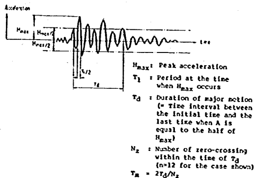
Fig. 2 Definition of Peak Acceleration, and Characteristic Variables of Strong-Motion Records
