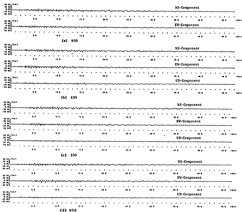
Fig. 48 Acceleration Records at N50, E50, S50 and W50 at Field-A of Local Laboratory Array of PWR1 in Tsukuba
