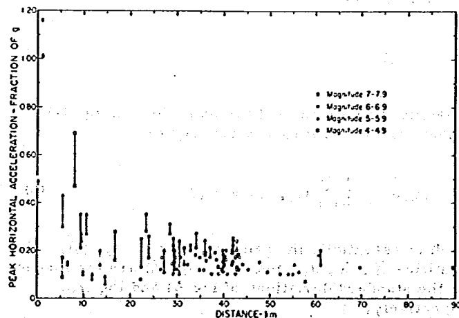
Fig. 8 Peak Acceleration vs. Distance for Four Magnitude Classes (Jennings and Helmberger (1978))
