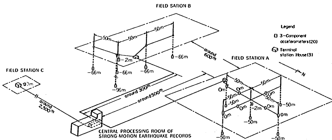
Fig. 43 Locations of Accelerometers of Local Laboratory Array at PWR1
