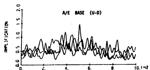
Fig. 35 FRF (Amplification) of A67 to E50 in Vertical (Tsuchida et al (1978))
