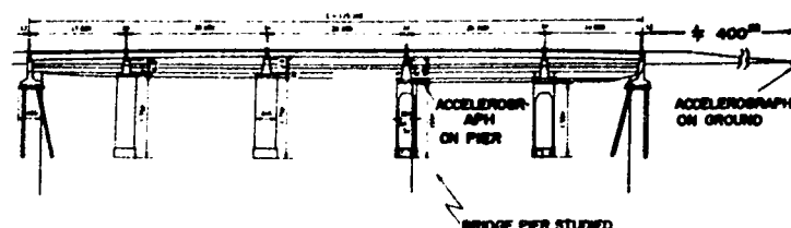
Fig. 65 General View of Itajima Bridge
