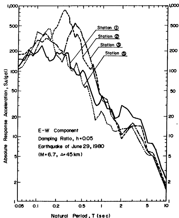
Fig. 61 Absolute Response Acceleration Spectra, E-W Components
