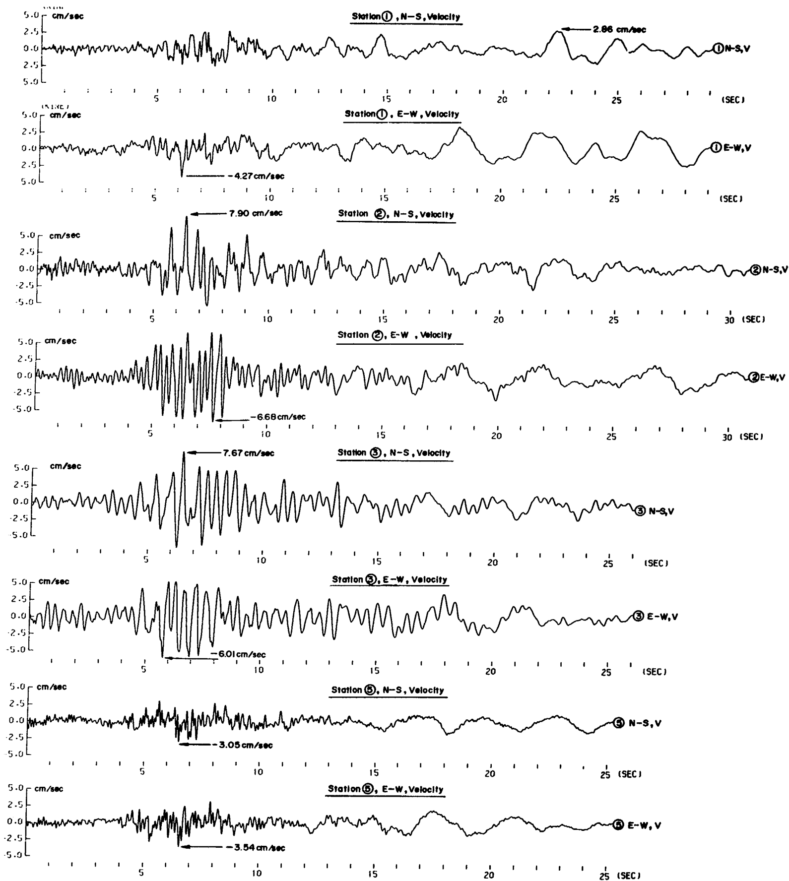
Fig. 57 Velocities Calculated from Acceleration Records at Four Stations During the Izu Peninsula Earthquake of June 29, 1980 (M=6.7, \Delta=45 km)
