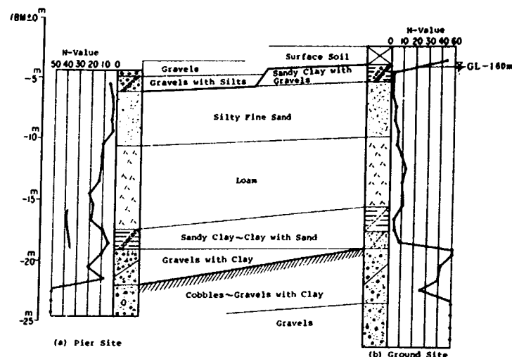
Fig. 66 Soil Profile at the Site of Itajima Bridge
