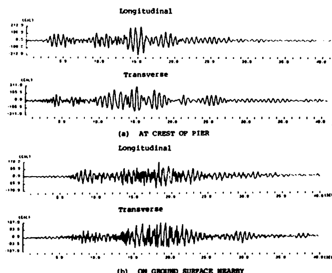
Fig. 67 Acceleration Records at Itajima Bridge During the Earthquake of April 1, 1968 ( M=7.5 )
