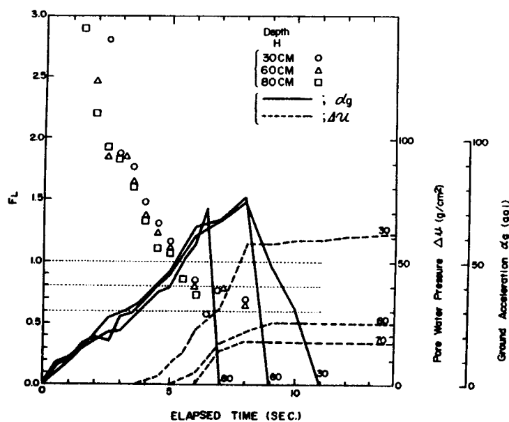
Fig. 9 Relationships between Pore Water Pressure and Acceleration of Liquefied Sand Layers and F_L Values in Shaking Table Tests
