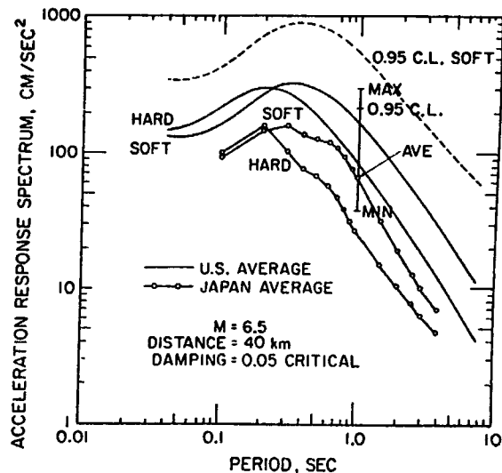
Fig. 21 Average Acceleration Response Spectrum Amplitudes for U.S. and Japanese Earthquakes (Hudson (1980))
