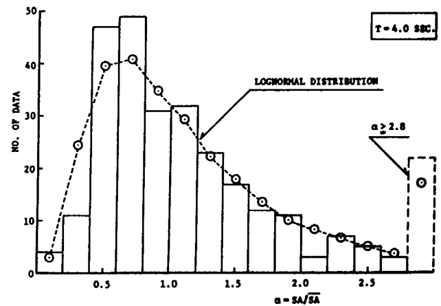
Fig. 19 Histogram of \alpha for T=4.0 sec
