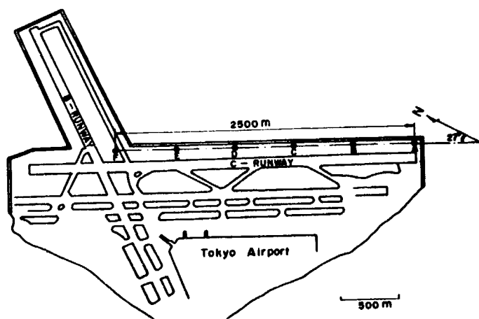
Fig. 23 Deployment of Accelerometers in Plan (Tsuchida et al (1978))
