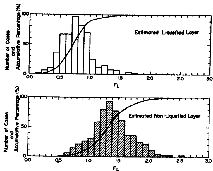
Fig. 6 Distribution of F_L Values and Their Accumulative Incidences, in Percentage, Comparing Liquefied Sites with Non-Liquefied Sites in Table 1
