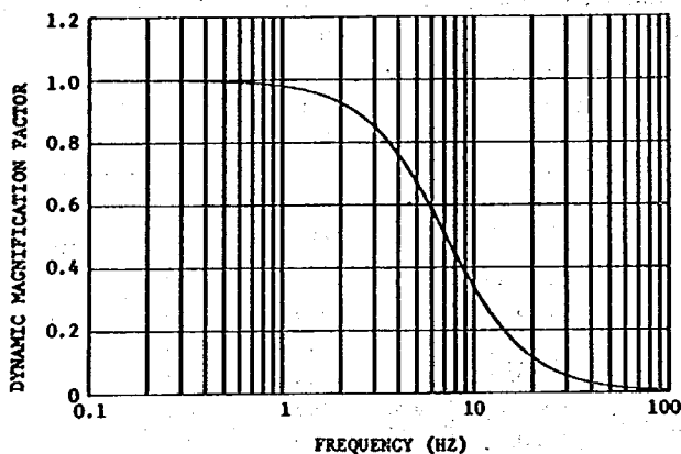
Fig. 4 Frequency Characteristics of SMAC-B2 Accelerograph
