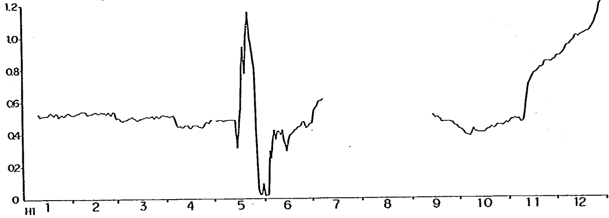
(g/cm 3 ) P-33(7.00m)
